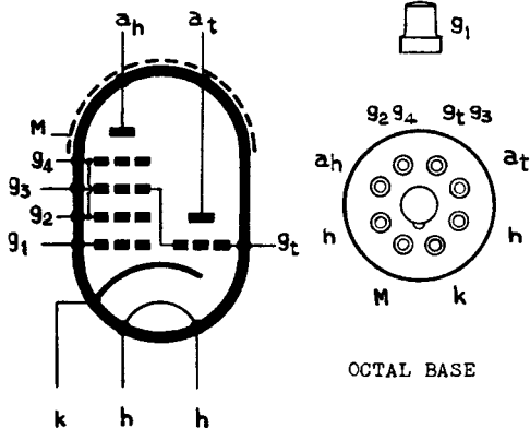
ARRANGEMENT OF ELECTRODES AND BASE CONNECTIONS
