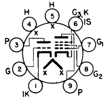
BOTTOM VIEW BASING DIAGRAM JEDEC 90X
