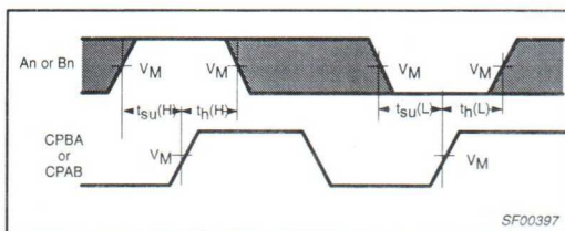
Waveform 4. Data Setup Time and Hold Times
