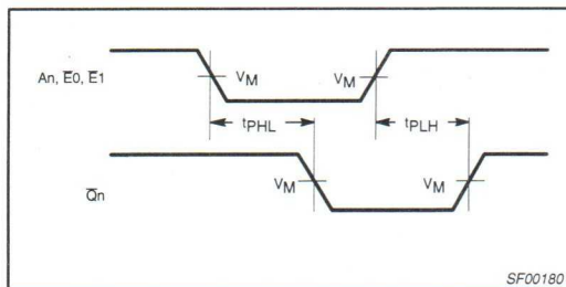
Waveform 2. Propagation Delay for Non-inverting Outputs
