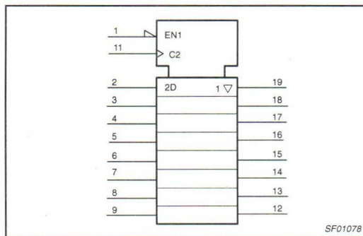
IEC/IEEE SYMBOL – 74ALS574A
