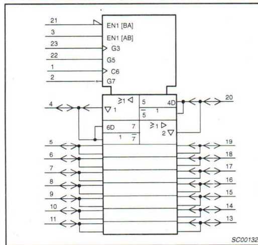
IEC/IEEE SYMBOL – 74ALS652/652-1
