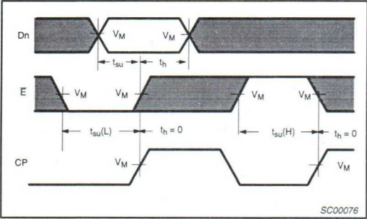
Waveform 2. Data and Enable Setup and Hold Times
