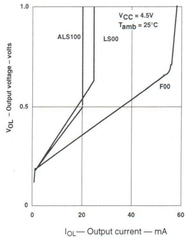
Figure 5. Output low characteristics
