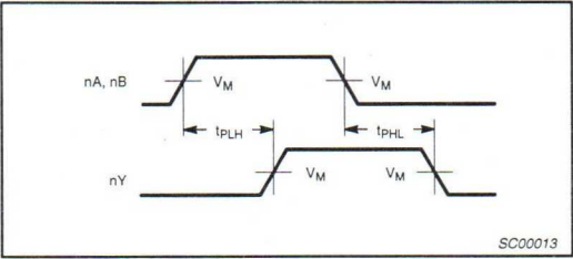
Waveform 2. Propagation Delay for Data to Output
