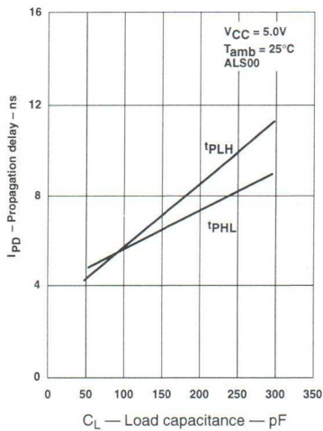
Figure 4. Propagation delay vs load capacitance
