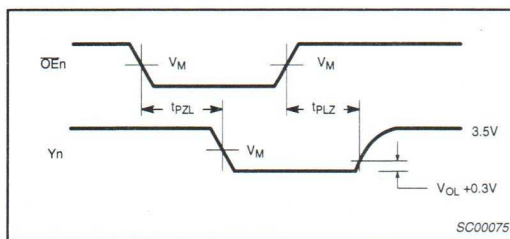
Waveform 3. 3-State Output Enable Time to Low Level and Output Disable Time from Low Level
