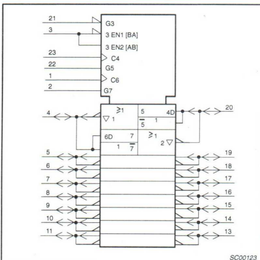
IEC/IEEE SYMBOL – 74ALS648/648-1
