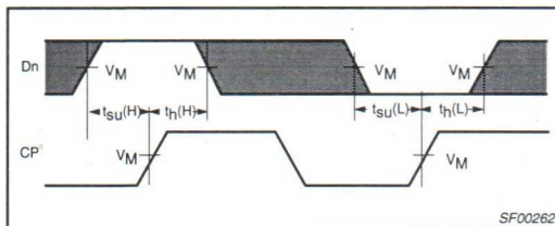
Waveform 5. Data Setup Time and Hold Times
