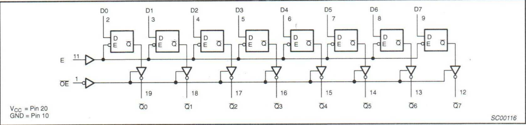
LOGIC DIAGRAM – 74ALS563A
