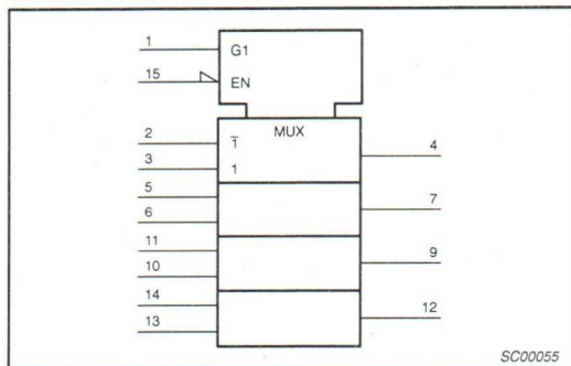
IEC/IEEE SYMBOL – 74ALS157
