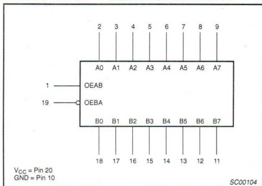
IEC/IEEE SYMBOL – 74ALS623A/74ALS623A-1
