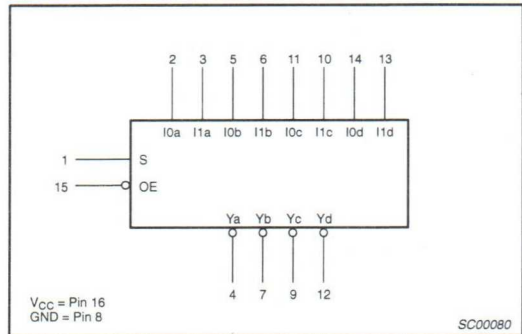
IEC/IEEE SYMBOL – 74ALS258
