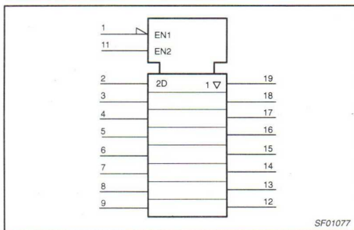
IEC/IEEE SYMBOL – 74ALS573B
