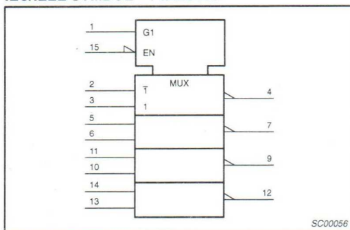
IEC/IEEE SYMBOL – 74ALS158
