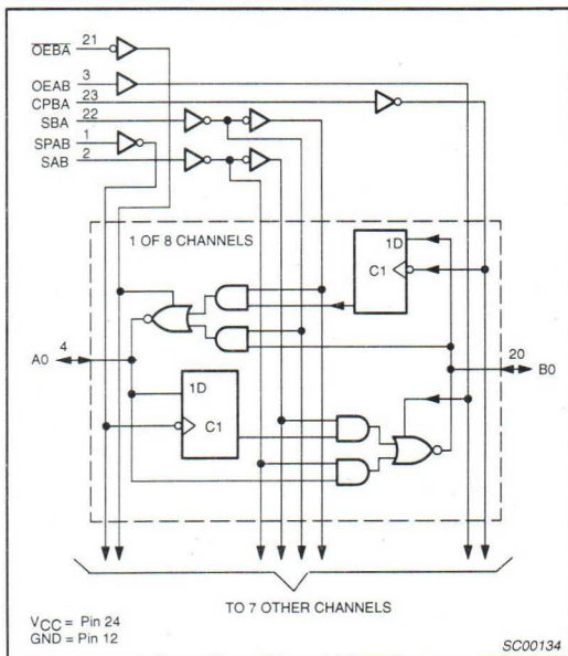
LOGIC DIAGRAM – 74ALS651/651-1
