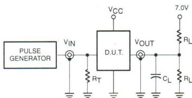
Test Circuit for Open Collector Outputs
