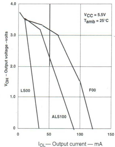
Figure 7. Output high characteristics
