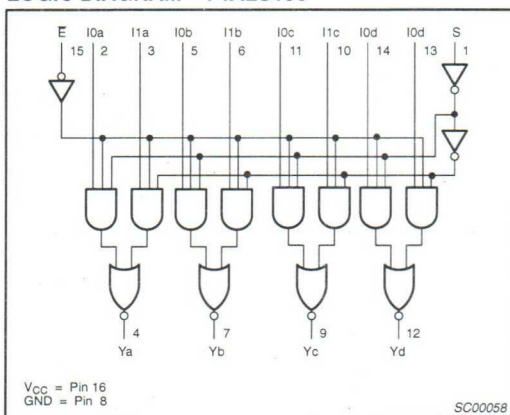
LOGIC DIAGRAM – 74ALS158
