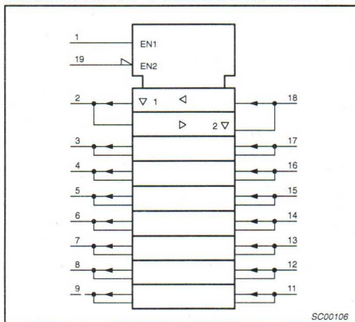
IEC/IEEE SYMBOL – 74ALS623A/74ALS623A-1
