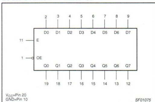
IEC/IEEE SYMBOL – 74ALS573B
