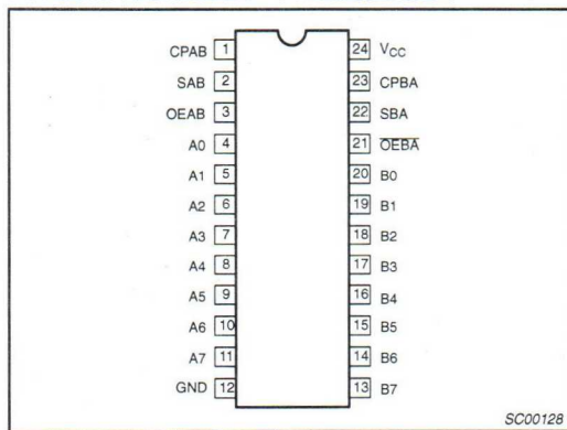
PIN CONFIGURATION – 74ALS652/652-1
