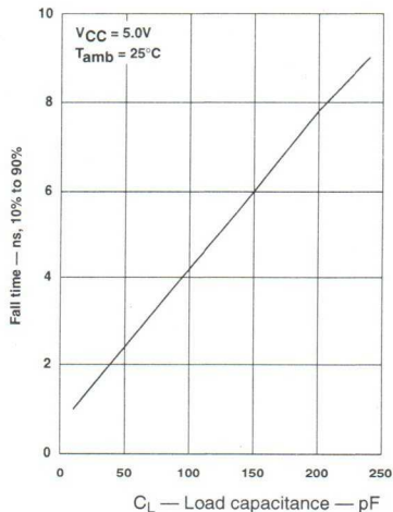
Figure 6. Fall time vs load capacitance
