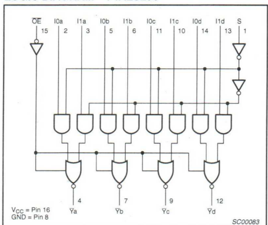
LOGIC DIAGRAM – 74ALS258
