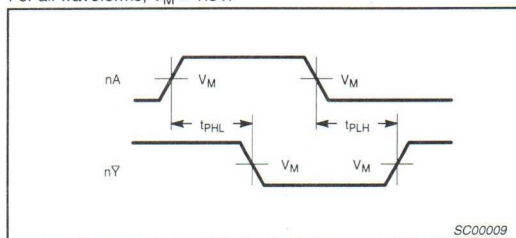
Waveform 1. Propagation Delay for Data to Output
