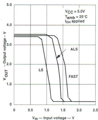
Figure 3. Transfer functions at room temperature
