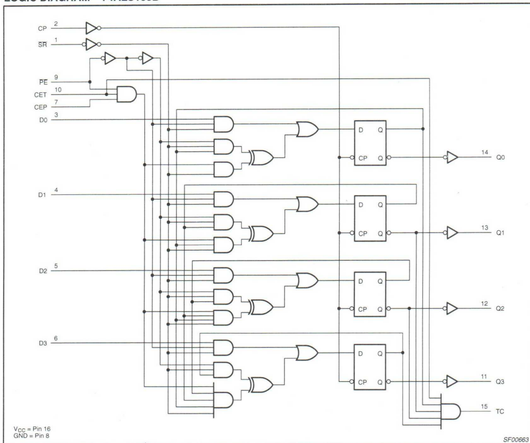
LOGIC DIAGRAM – 74ALS163B
