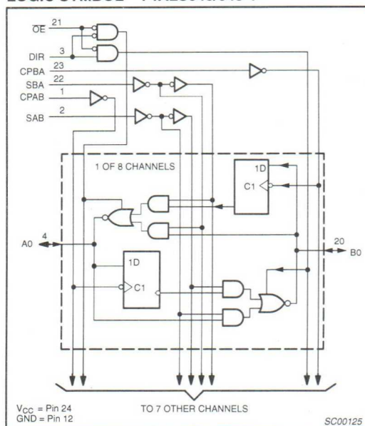
LOGIC SYMBOL – 74ALS648/648-1
