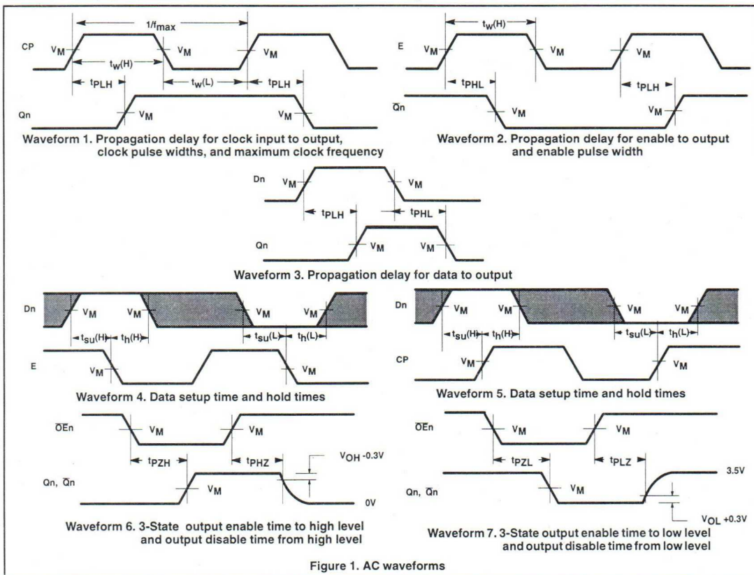
Figure 1. AC waveforms
