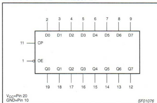
IEC/IEEE SYMBOL – 74ALS574A
