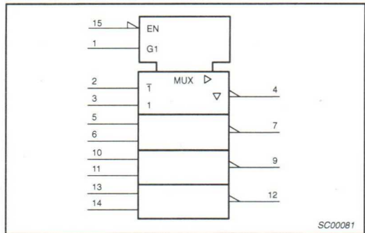
LOGIC DIAGRAM – 74ALS258
