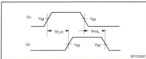
Waveform 3. Propagation Delay for Data to Output
