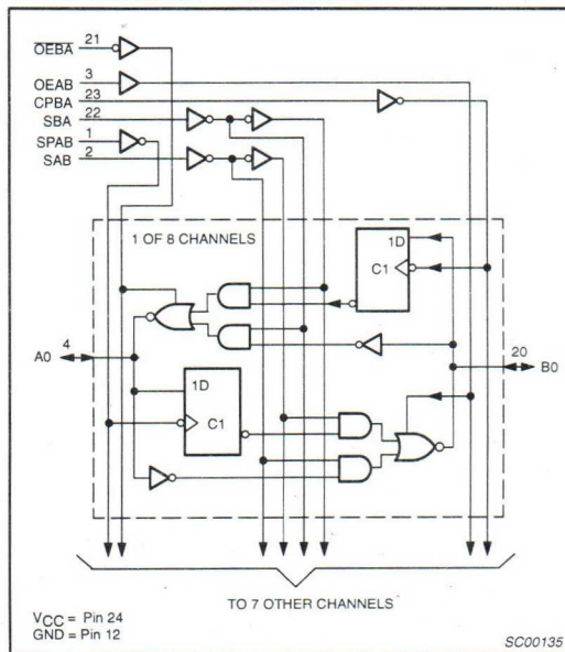
LOGIC DIAGRAM – 74ALS652/652-1
