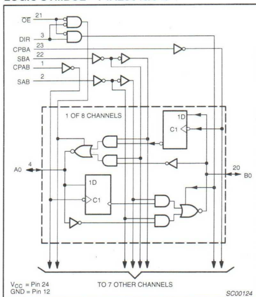
LOGIC SYMBOL – 74ALS646/646-1
