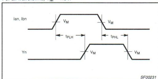
Waveform 1. Propagation Delay for Non-inverting Outputs
