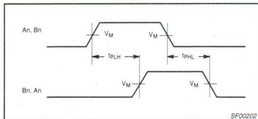
Waveform 2. Propagation Delay for Non-inverting Outputs
