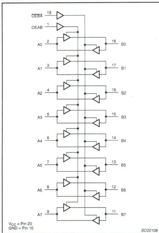
LOGIC DIAGRAM – 74ALS623A/74ALS623A-1
