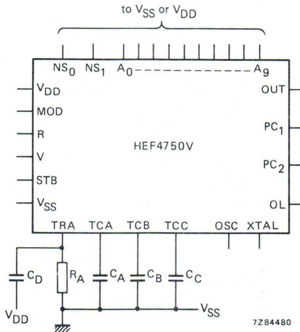
Fig. 8 Test circuit for measuring a.c. characteristics.
