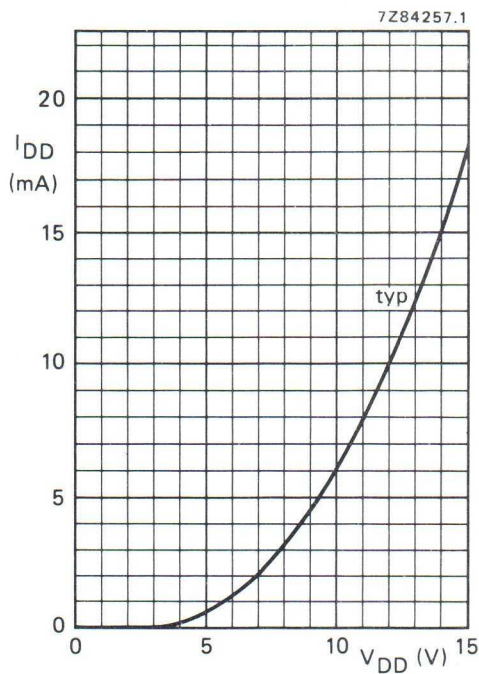
Fig. 5 Supply current as a function of supply voltage.
