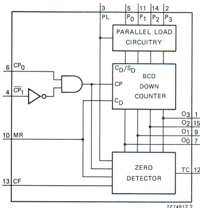
Fig. 1 Functional diagram.
