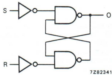
Fig. 4 Logic diagram (one latch).
