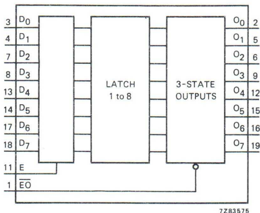
Fig. 1 Functional diagram.
