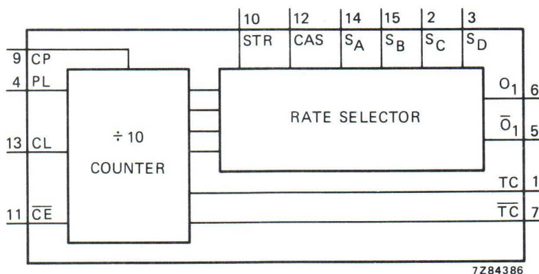
Fig. 1 Functional diagram.
