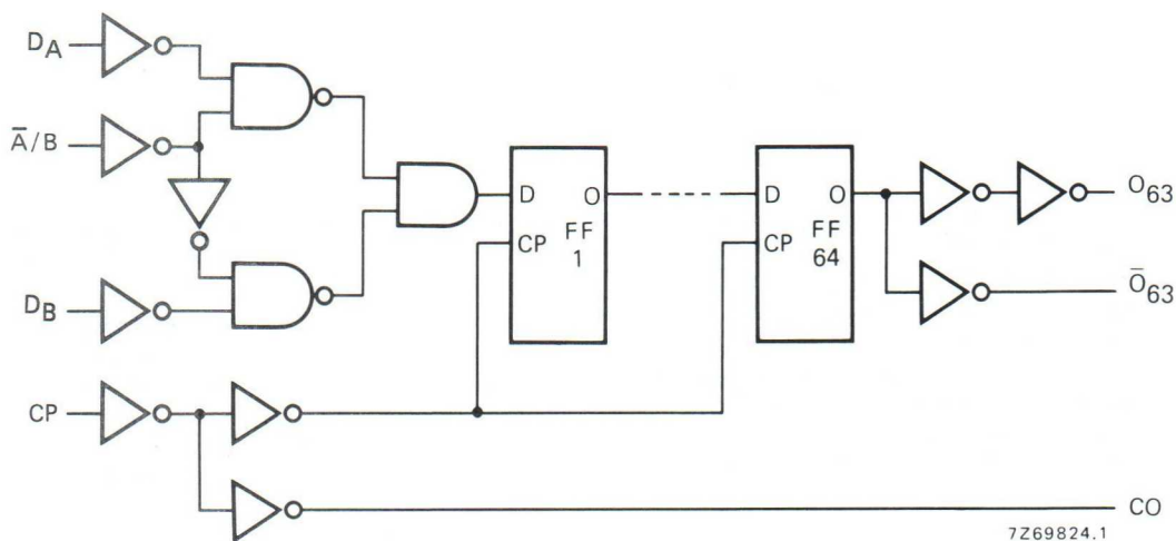
Fig. 3 Logic diagram.
