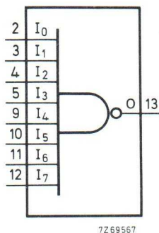
Fig. 1 Functional diagram.
