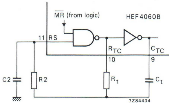
Fig. 4 External component connection for RC oscillator.
