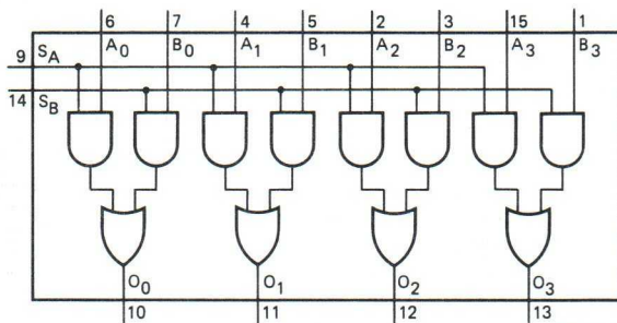
Quadruple 2-input multiplexer.
