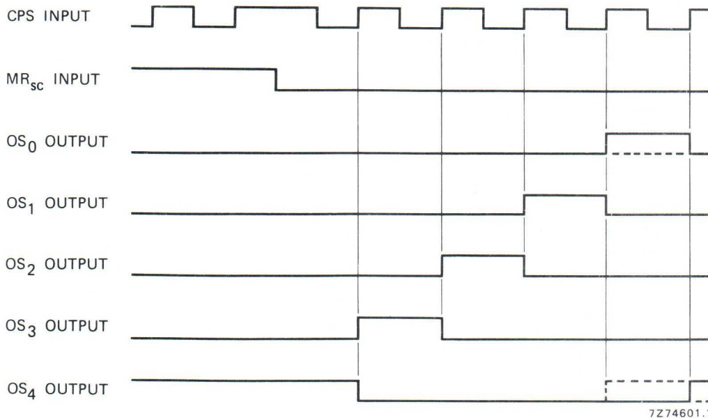
Fig. 7 Scanner timing diagram.
