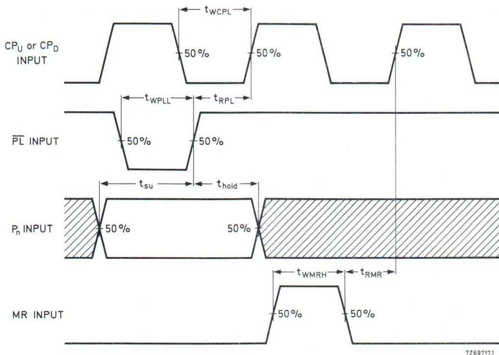
Fig. 5 Waveforms showing recovery times for \overline{PL} and MR, minimum pulse widths for CP U , CP D , \overline{PL} and MR, and set-up and hold times for P to \overline{PL} . Set-up times and hold times are shown as positive values but may be specified as negative values.
