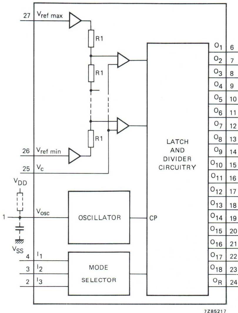
Fig. 1 Functional diagram.
