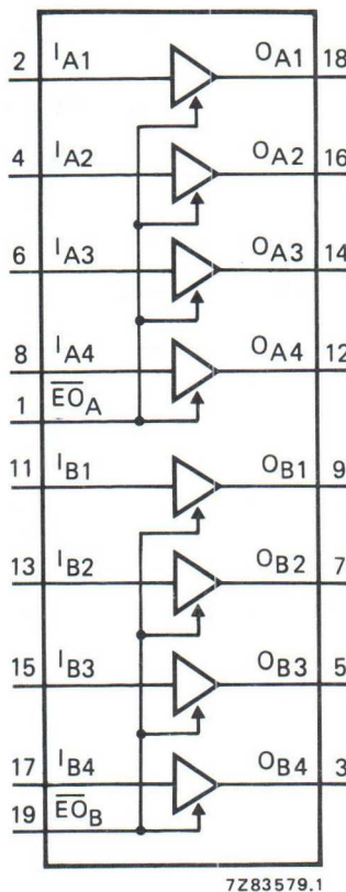
Fig. 1 Functional diagram.
