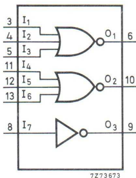
Fig. 1 Functional diagram.
