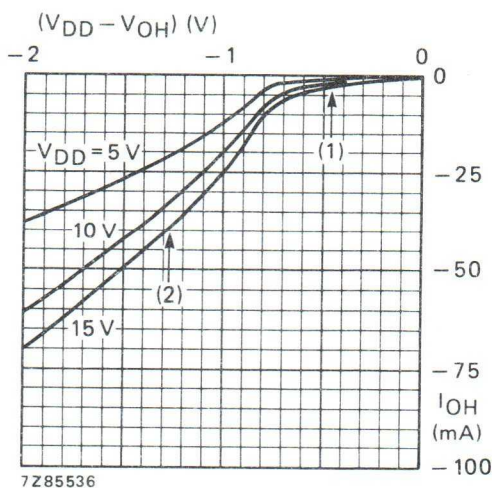
Fig. 5 Typical output source current characteristic.
