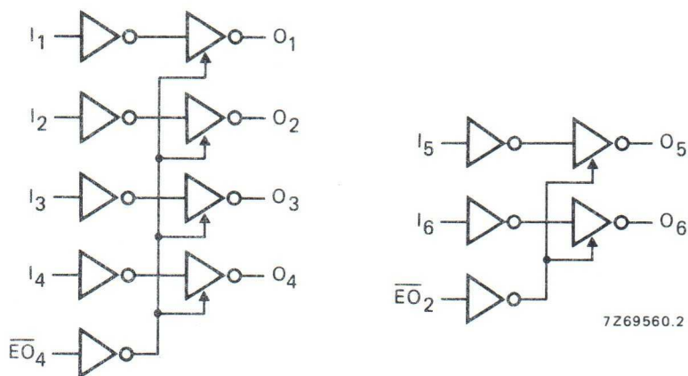
Fig. 3 Logic diagram.
