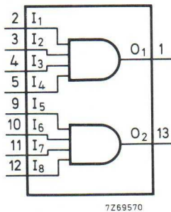
Fig. 1 Functional diagram.
