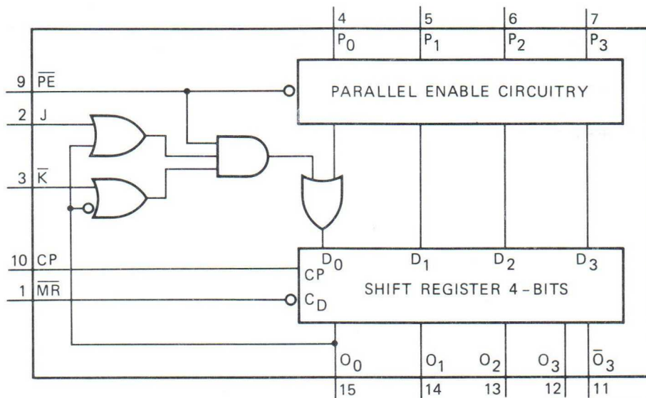
Fig. 1 Functional diagram.
