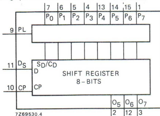
Fig. 1 Functional diagram.
