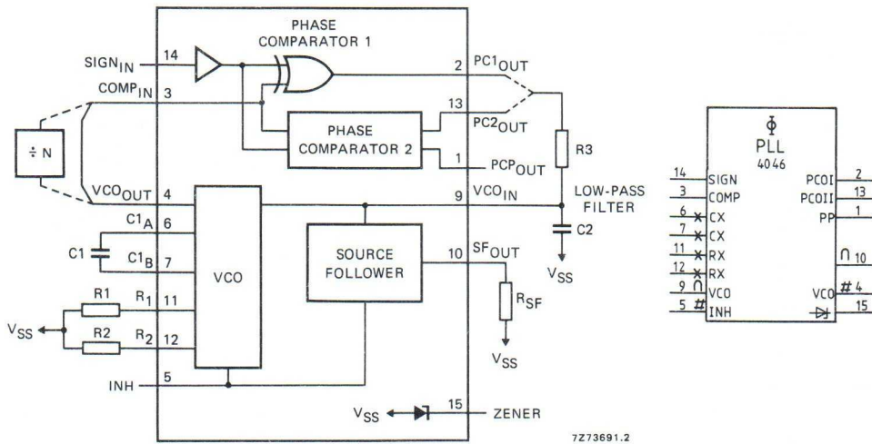
Phase-locked loop.
