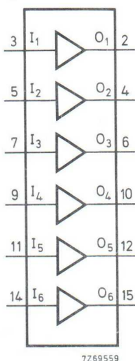
Fig. 1 Functional diagram.
