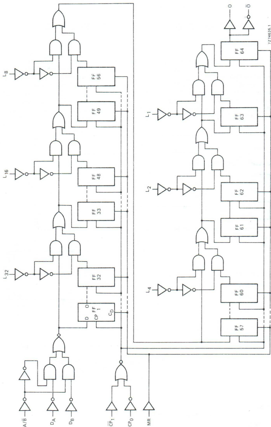
Fig. 3 Logic diagram.
