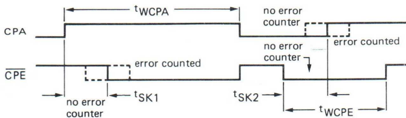
Fig. 4 Skew times timing diagram; t_{WCPA} > t_{SK1} ; t_{WCE} > t_{SK2} .
