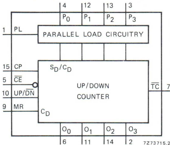
Fig. 1 Functional diagram.
