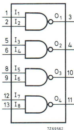
Fig. 1 Functional diagram.
