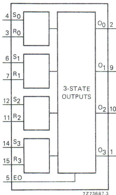
Fig. 1 Functional diagram.
