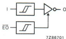
Fig. 3 Logic diagram (one buffer).
