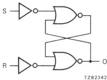
Fig. 4 Logic diagram (one latch).
