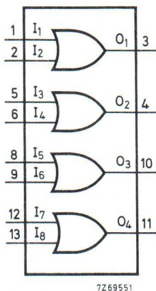
Fig. 1 Functional diagram.
