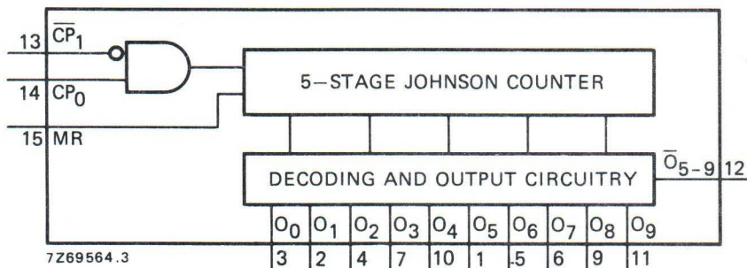
Fig. 1 Functional diagram.
