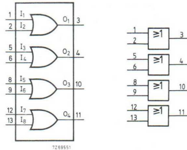
Quaduple 2-input OR gate.
