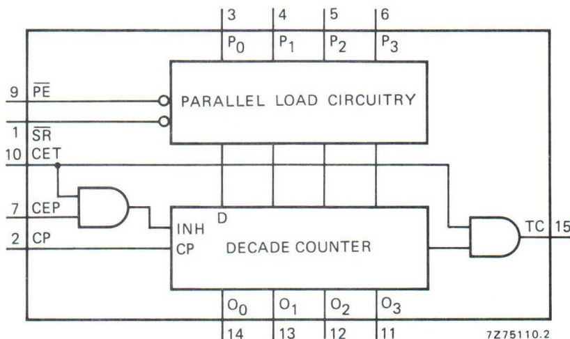
Fig. 1 Functional diagram.
