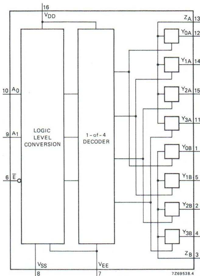
Fig. 1 Functional diagram.
