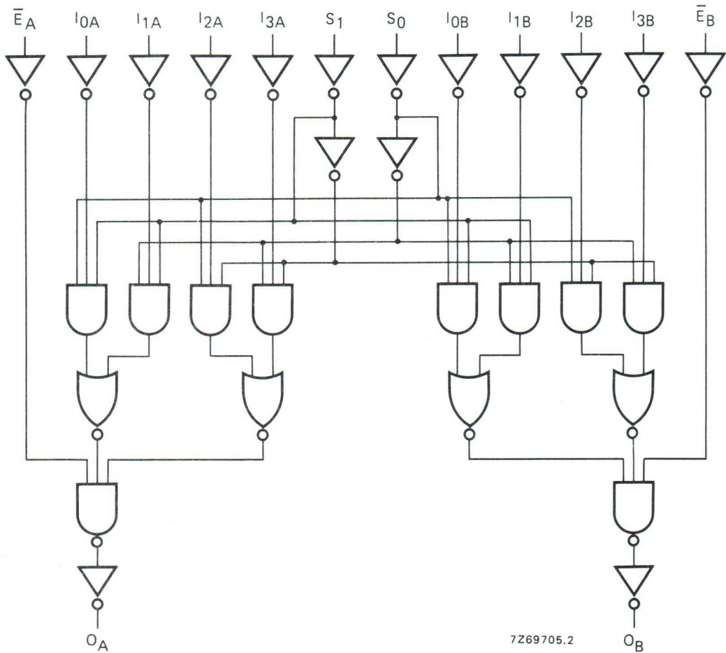
Fig. 3 Logic diagram.
