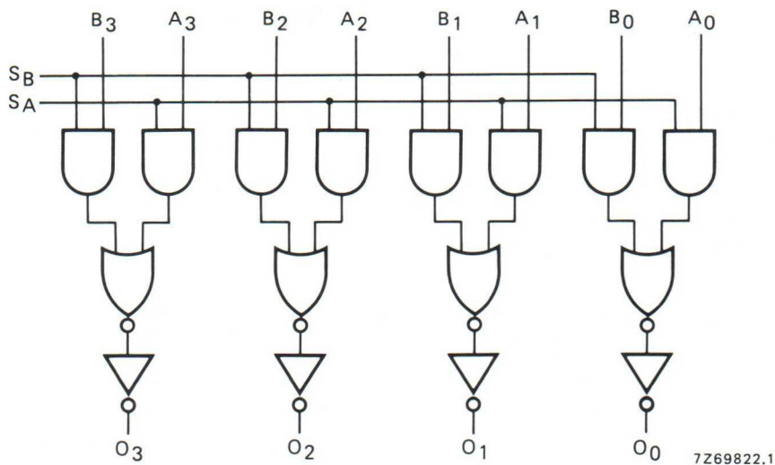
Fig. 3 Logic diagram.
