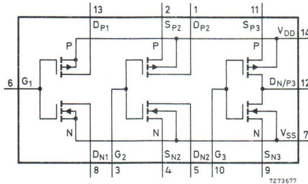
Fig. 1 Schematic diagram.
