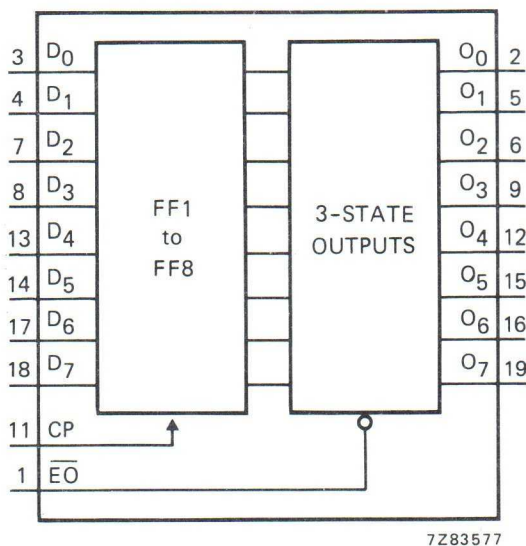
Fig. 1 Functional diagram.
