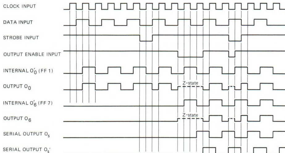
Fig. 4 Timing diagram.
