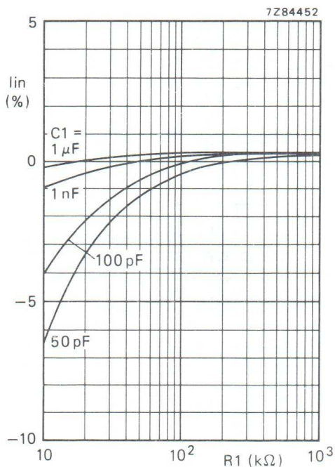
Fig. 15 VCO frequency linearity as a function of R1 ; R2 = \infty ; V_{DD} = 10 V .
