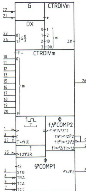
Frequency synthesizer.
