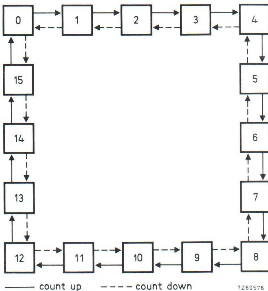
Fig. 5 State diagram; \text{BIN}/\overline{\text{DEC}} = \text{HIGH} .
