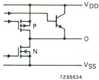
Fig. 5 Schematic diagram of output stage.
