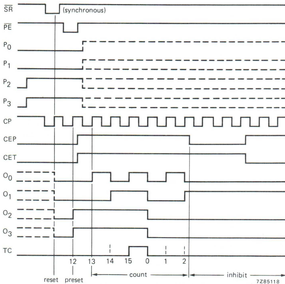
Fig. 9 Timing diagram.
