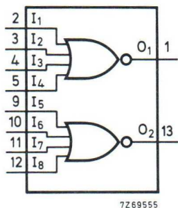
Fig. 1 Functional diagram.
