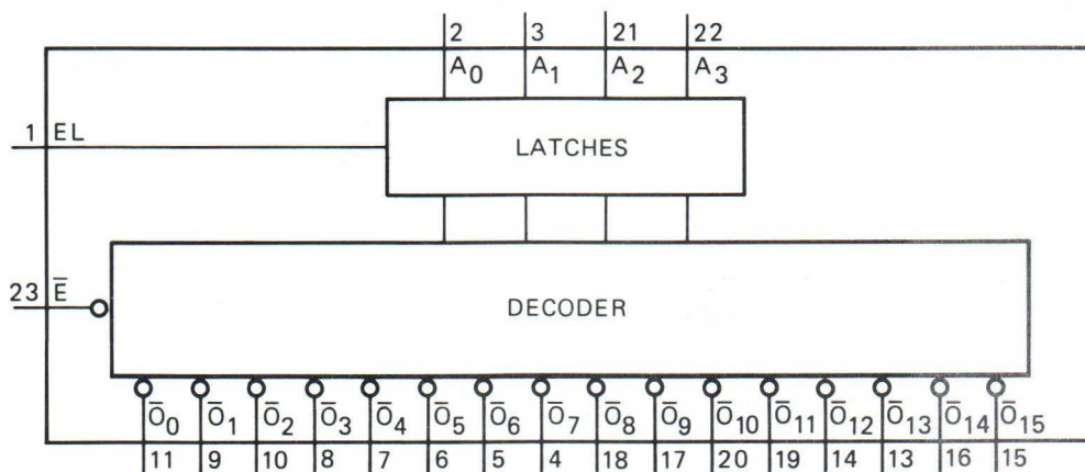
Fig. 1 Functional diagram.
