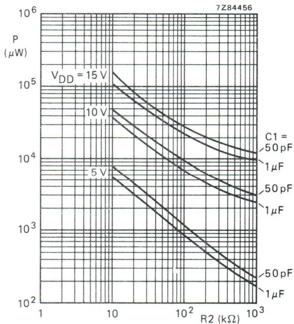
Fig. 11 Power dissipation as a function of R_2 ; R_1 = \infty ; V_{COIN} at V_{SS} (0 V); C_L = 50 pF .
