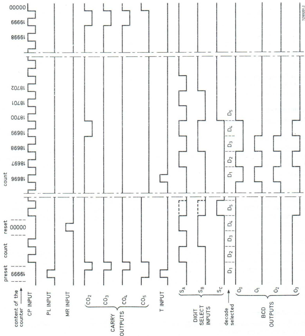
Fig. 3 Timing diagram.
