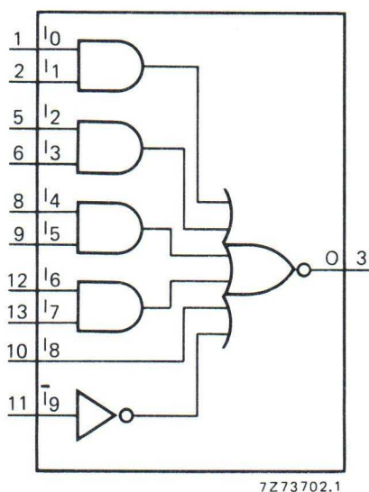
Fig. 1 Functional diagram.
