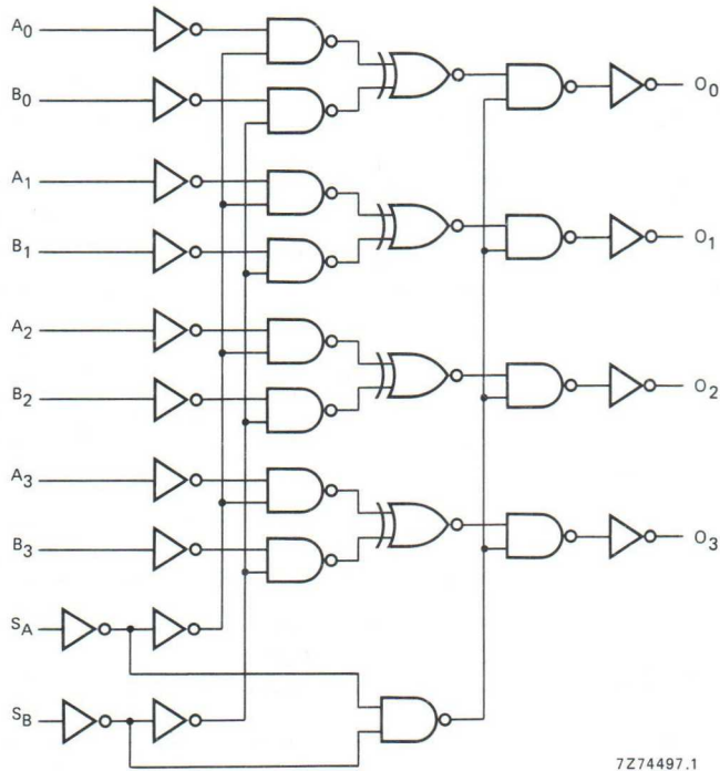
Fig. 3 Logic diagram.
