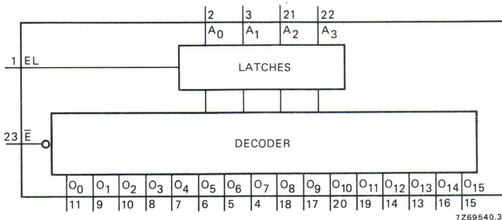
Fig. 1 Functional diagram.
