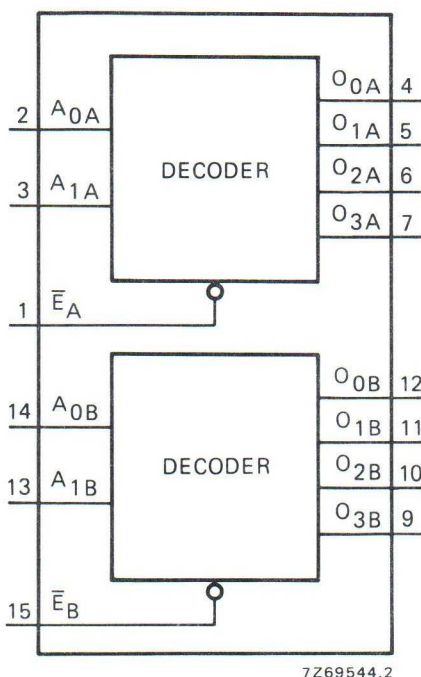
Fig. 1 Functional diagram.
