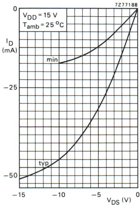
P-channel drain characteristics (source)
