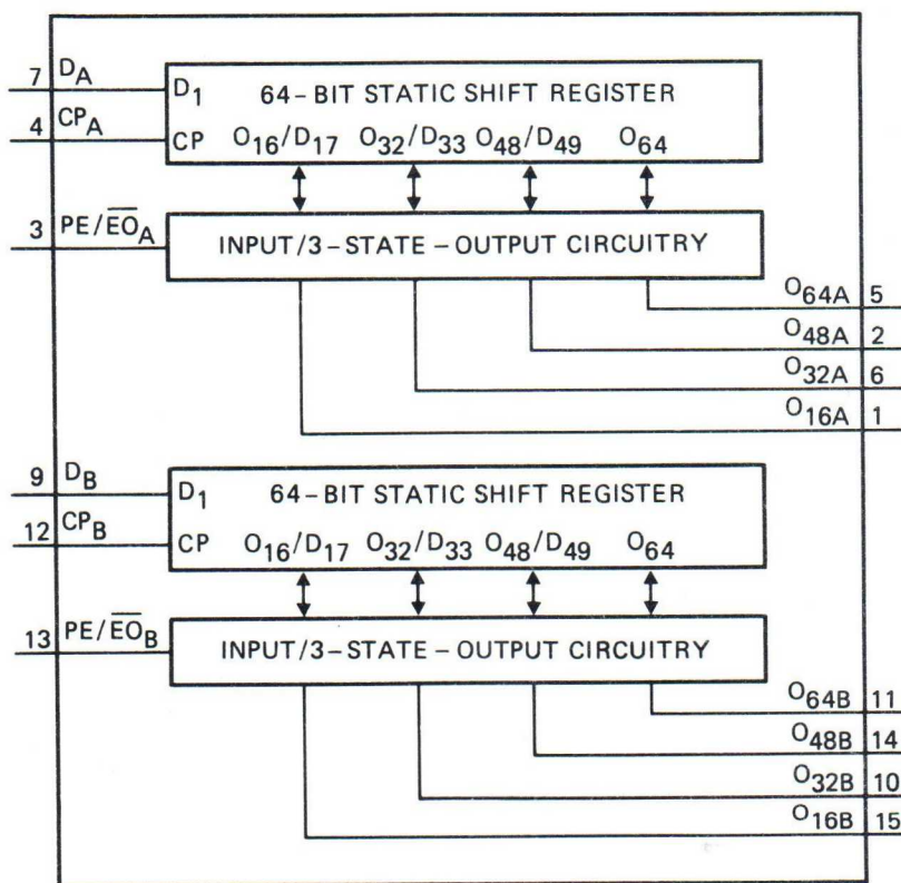
Fig. 1 Functional diagram.
