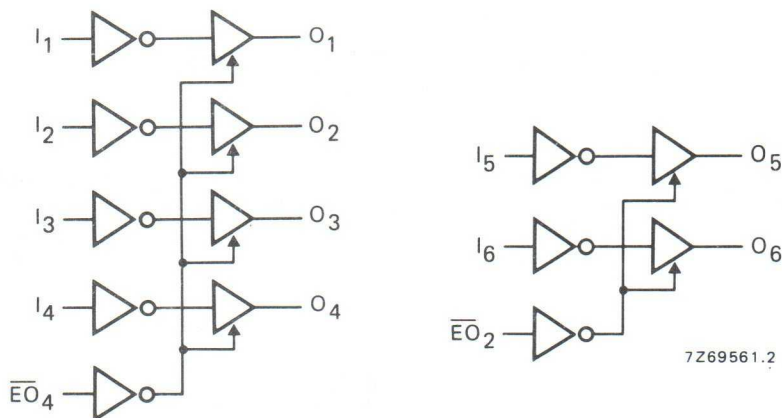
Fig. 3 Logic diagram.
