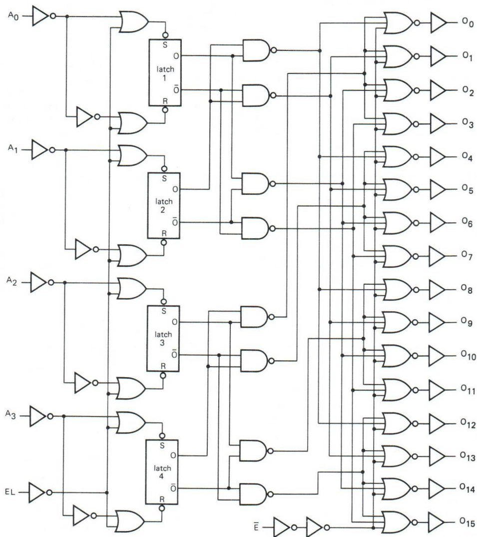
Fig. 3 Logic diagram.
