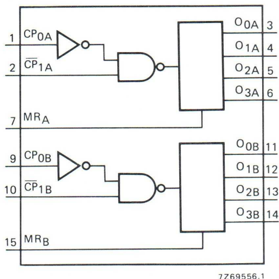
Fig. 1 Functional diagram.
