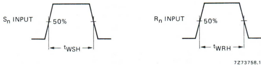
Fig. 5 Waveforms showing minimum S_n and R_n pulse widths.
