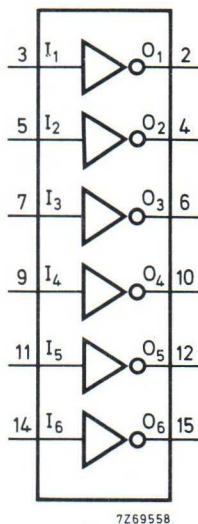
Fig. 1 Functional diagram.
