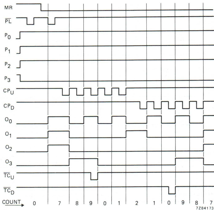
Fig. 6 Timing diagram.
