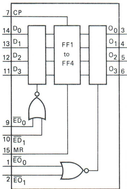
Fig. 1 Functional diagram.
