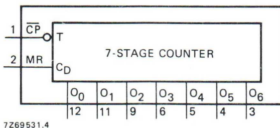
Fig. 1 Functional diagram.
