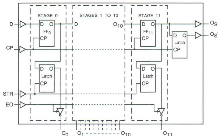
Fig.3 Logic diagram.
