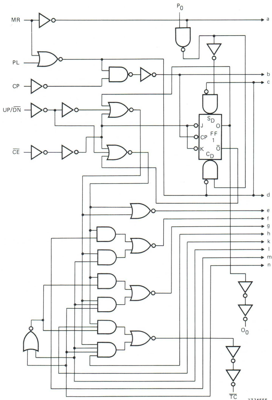
Fig. 3a Logic diagram (continued in Fig. 3b).
