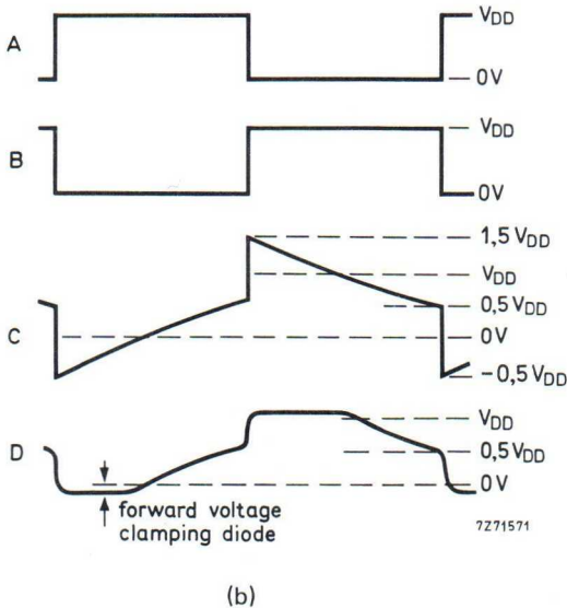
Fig. 9(a) Astable relaxation oscillator using two HEF4011UB gates; the diodes may be BAW62; C2 is a parasitic capacitance. (b) Waveforms at the points marked A, B, C and D in the circuit diagram.
