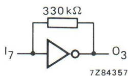
Fig. 6 Test set-up for measuring graphs of Figs 4 and 5.
