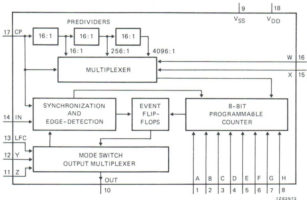
Fig. 1 Functional diagram.
