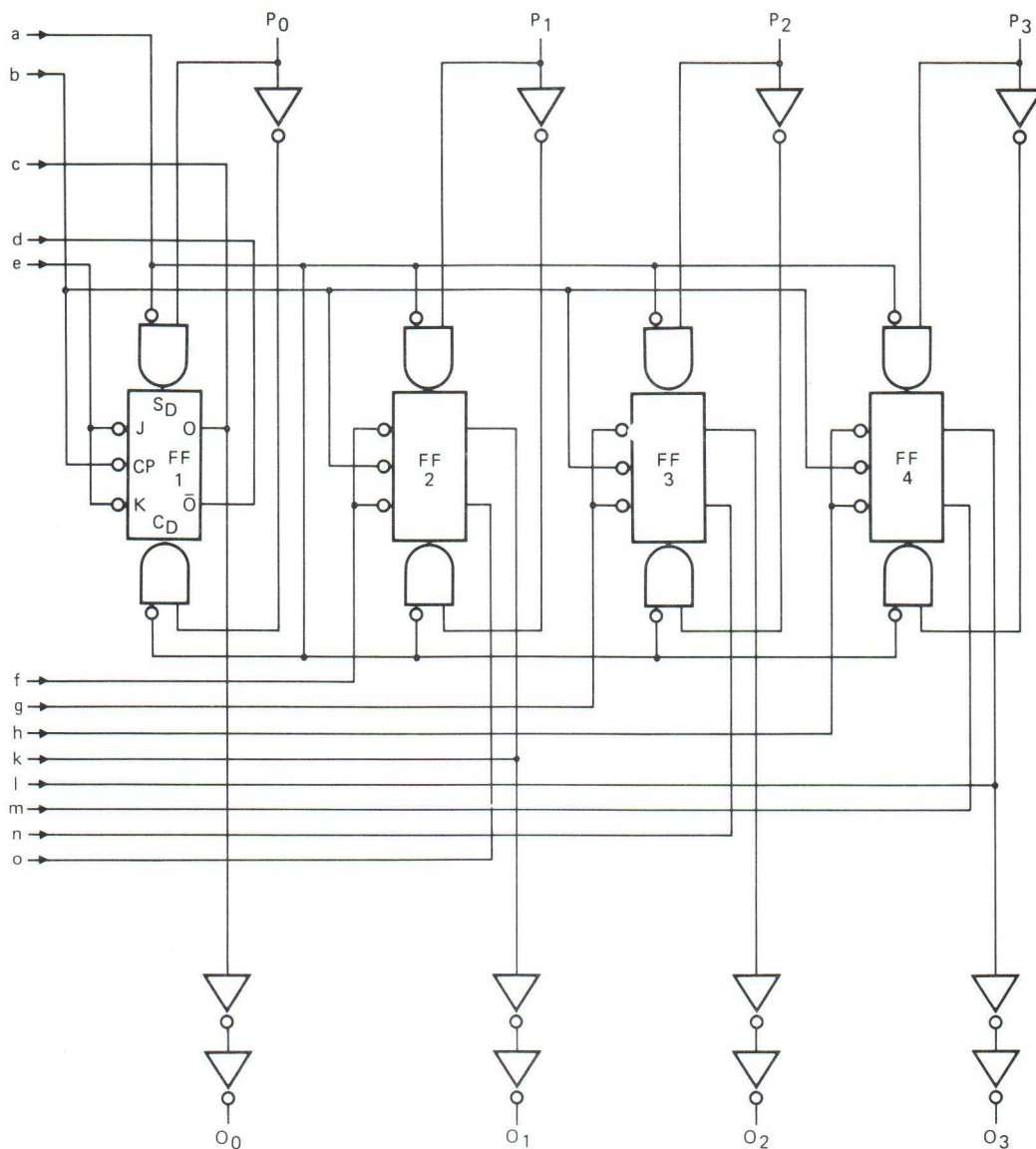
Fig. 3b Logic diagram (continued from Fig. 3a).
