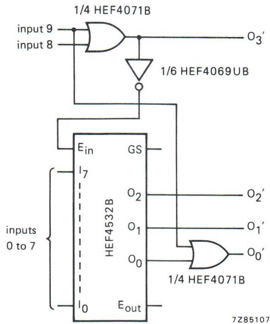
Fig. 6 0-to-9 keyboard encoder.
