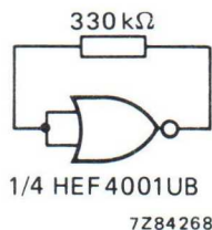
Fig. 15 Test set-up for measuring graphs of Figs 13 and 14. Condition: all other inputs connected to ground.
