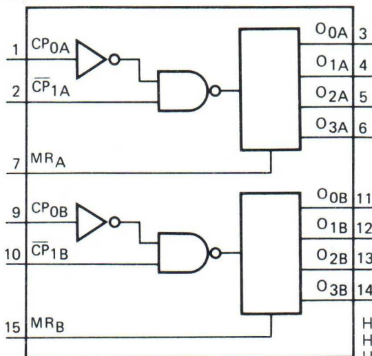
Fig. 1 Functional diagram.
