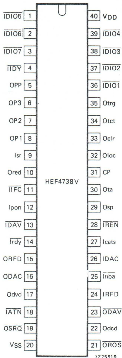
Fig. 2 Pinning diagram; for abbreviations see the following list.
