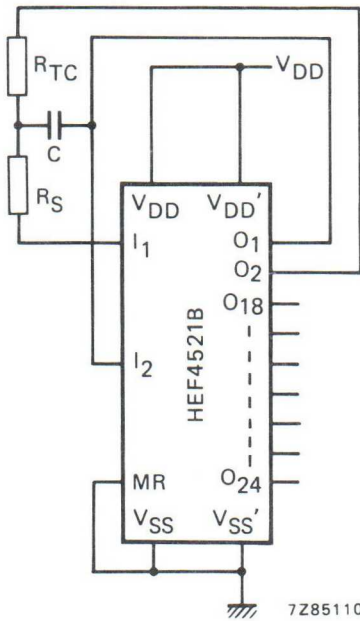
Fig. 7 RC oscillator circuit;
