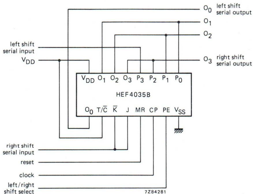
Fig. 6 Shift-left/shift-right register.
