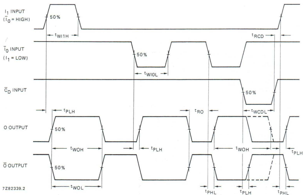
Fig. 5 Waveforms showing minimum \bar{I}_0 , I_1 , O and \bar{C}_0 pulse widths, recovery times and propagation delays.
