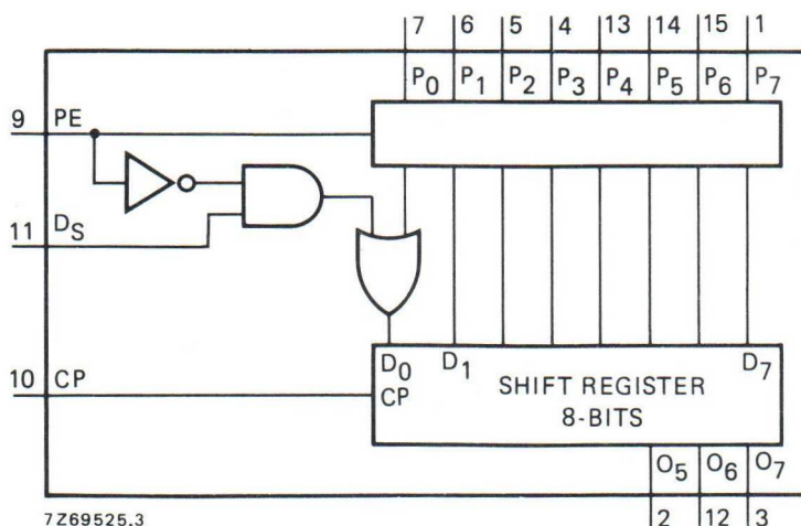
Fig. 1 Functional diagram.
