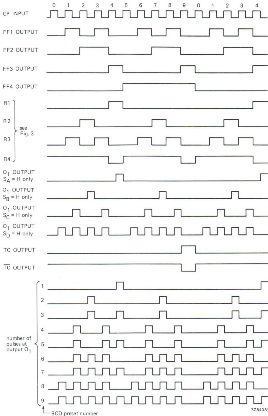
Fig. 4 Timing diagram.
