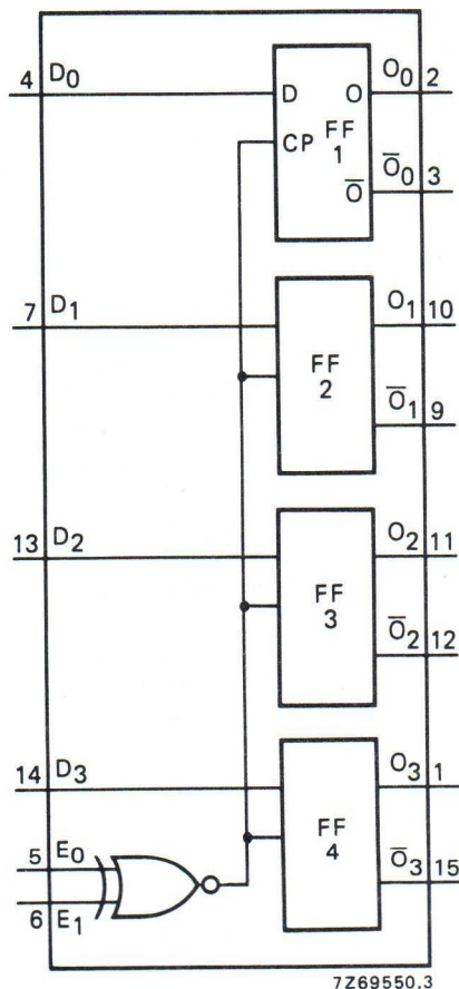
Fig. 1 Functional diagram.
