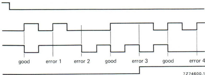
Fig. 3 Error detection timing diagram.
