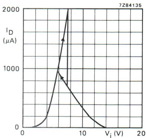
Fig. 8 Typical drain current as a function of input voltage; V_{DD} = 15\text{ V} ; T_{amb} = 25^\circ\text{C} .
