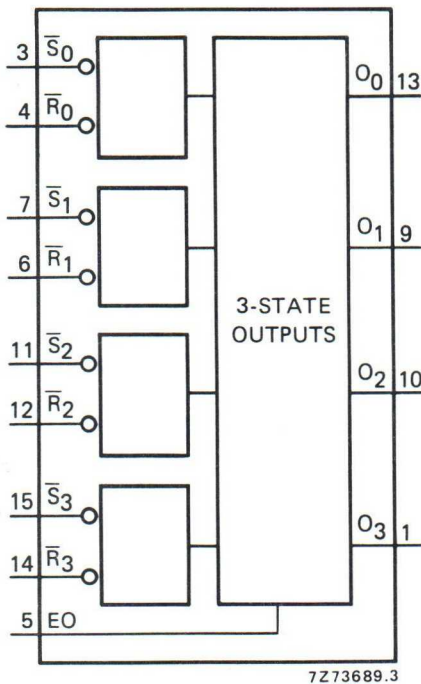
Fig. 1 Functional diagram.
