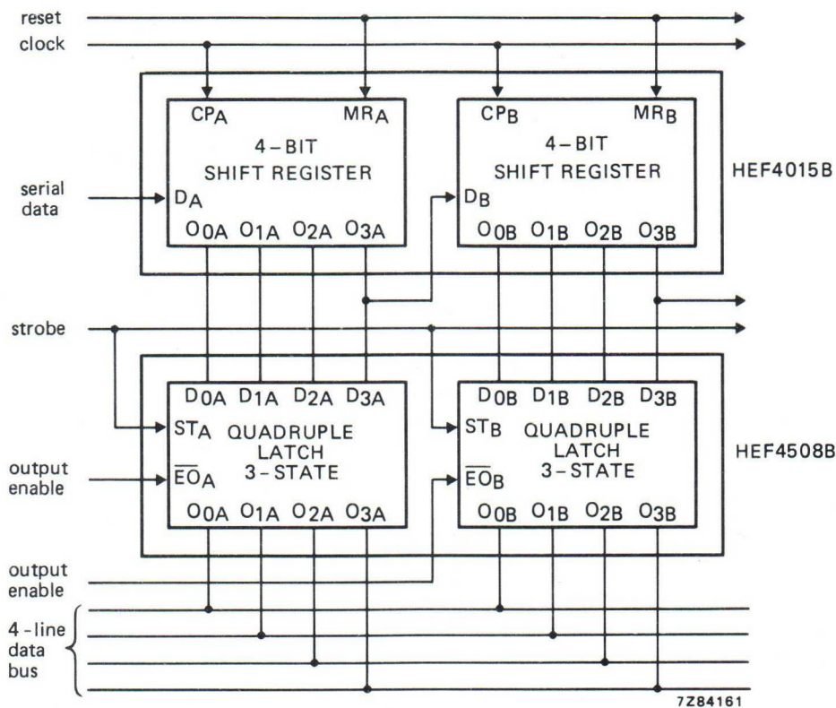
Fig. 5 Example of a bus register using HEF4508B and HEF4015B.
