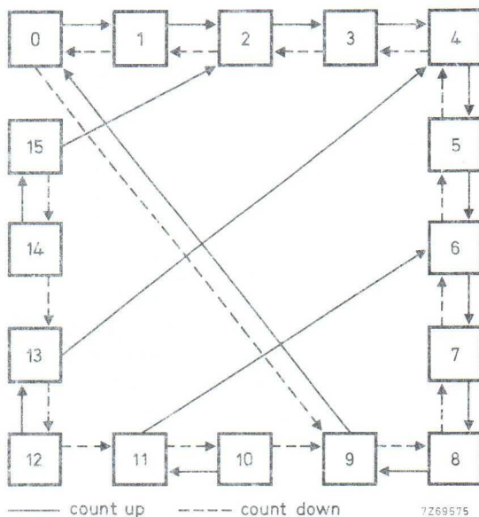
Fig. 4 State diagram.
