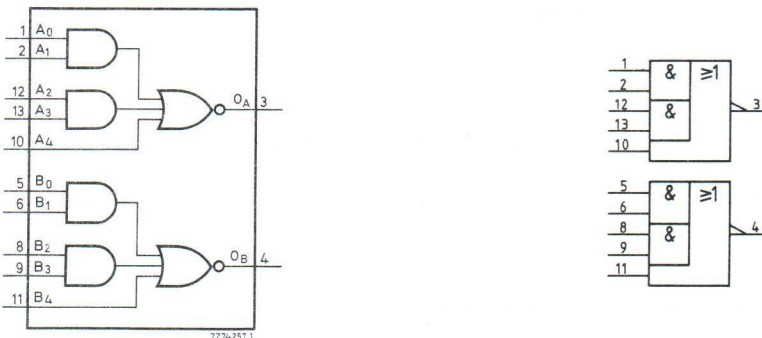
Dual 2-wide 2-input AND-OR-INVERT gate.
