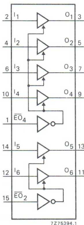
Fig. 1 Functional diagram.
