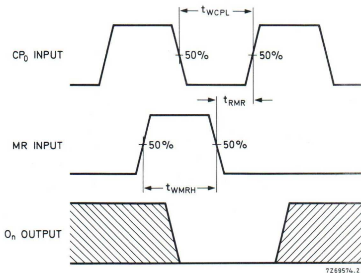
Fig. 5 Waveforms showing recovery time for MR; minimum CP_0 and MR pulse widths. Conditions: \overline{CP}_1 = \text{LOW} while CP_0 is triggered on a LOW to HIGH transition. t_{WCPH} and t_{RMR} also apply when CP_0 = \text{HIGH} and \overline{CP}_1 is triggered on a HIGH to LOW transition.
