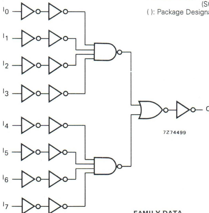
Fig. 3 Logic diagram.
