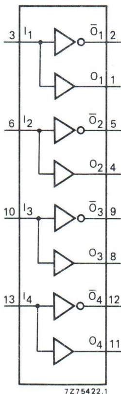
Fig. 1 Functional diagram.
