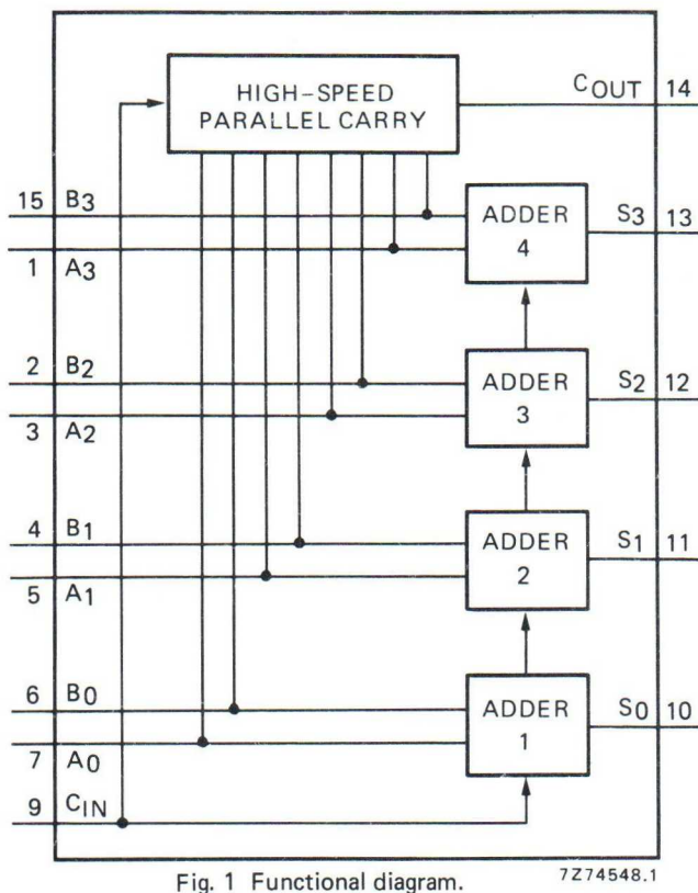
Fig. 1 Functional diagram.
