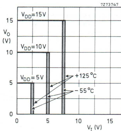
Fig. 12 Voltage transfer characteristic over -55 to +125 °C range.
