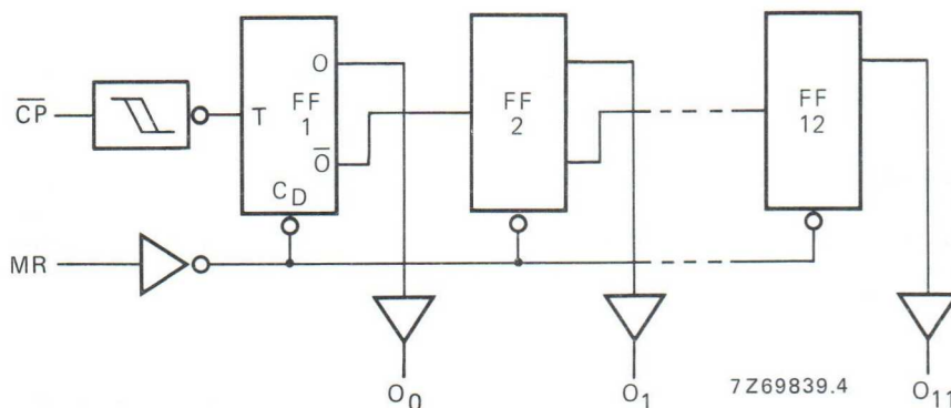
Fig. 3 Logic diagram.
