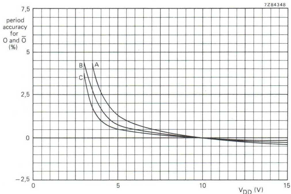
Fig. 5 Typical O and \bar{O} period accuracy as a function of supply voltage; astable mode; T_{amb} = 25^{\circ}\text{C} .
