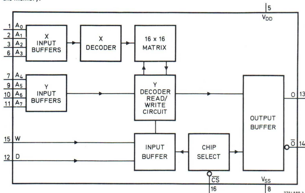
Fig. 1 Functional diagram.
