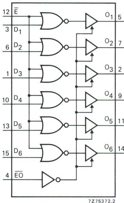
Fig. 1 Functional diagram.
