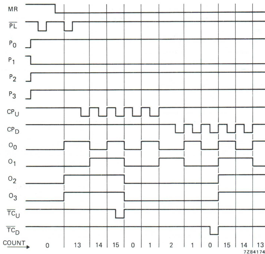
Fig. 6 Timing diagram.
