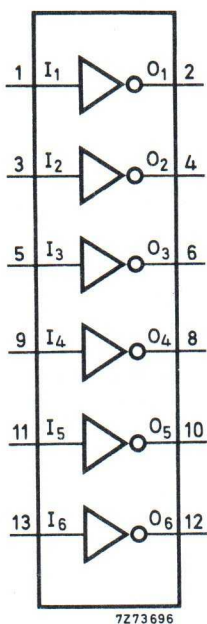
Fig. 1 Functional diagram.
