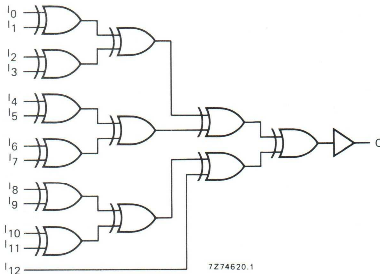
Fig. 3 Logic diagram.
