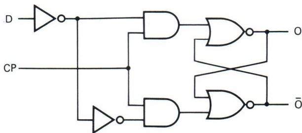
Fig. 6 Logic diagram (one latch); see also Fig. 5.
