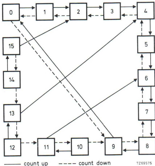
Fig. 4 State diagram; \text{BIN}/\overline{\text{DEC}} = \text{LOW} .
