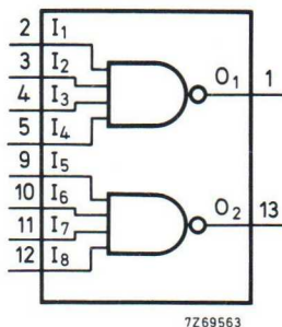
Fig. 1 Functional diagram.
