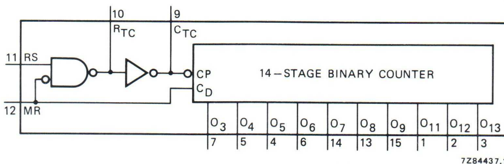
Fig. 1 Functional diagram.
