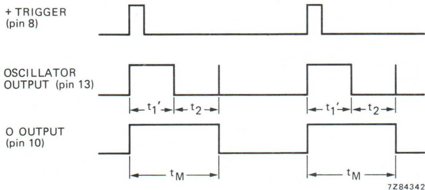
Fig. 7 Monostable waveforms.
