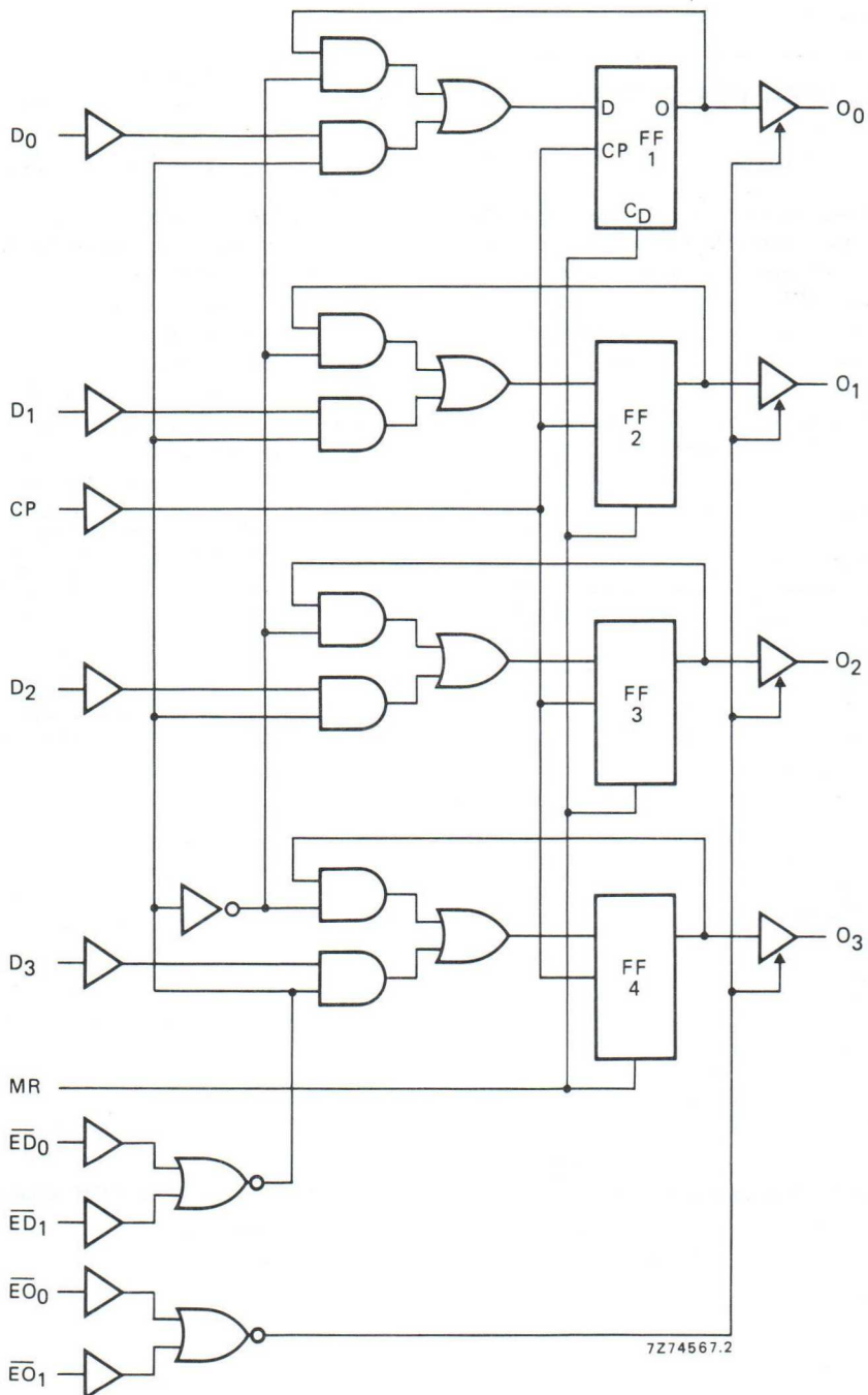
Fig. 3 Logic diagram.
