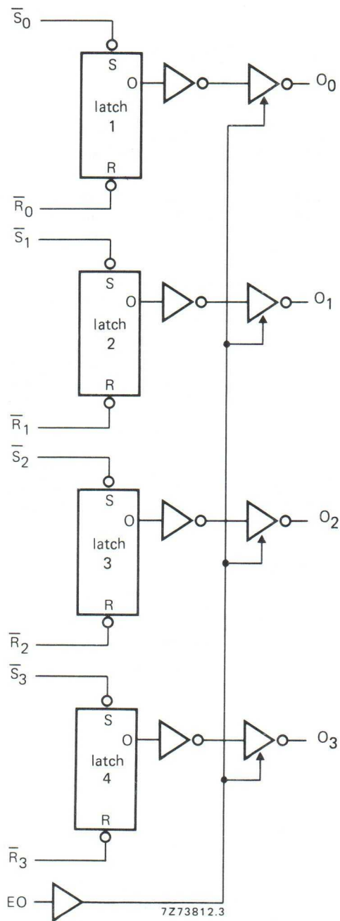
Fig. 3 Logic diagram.
