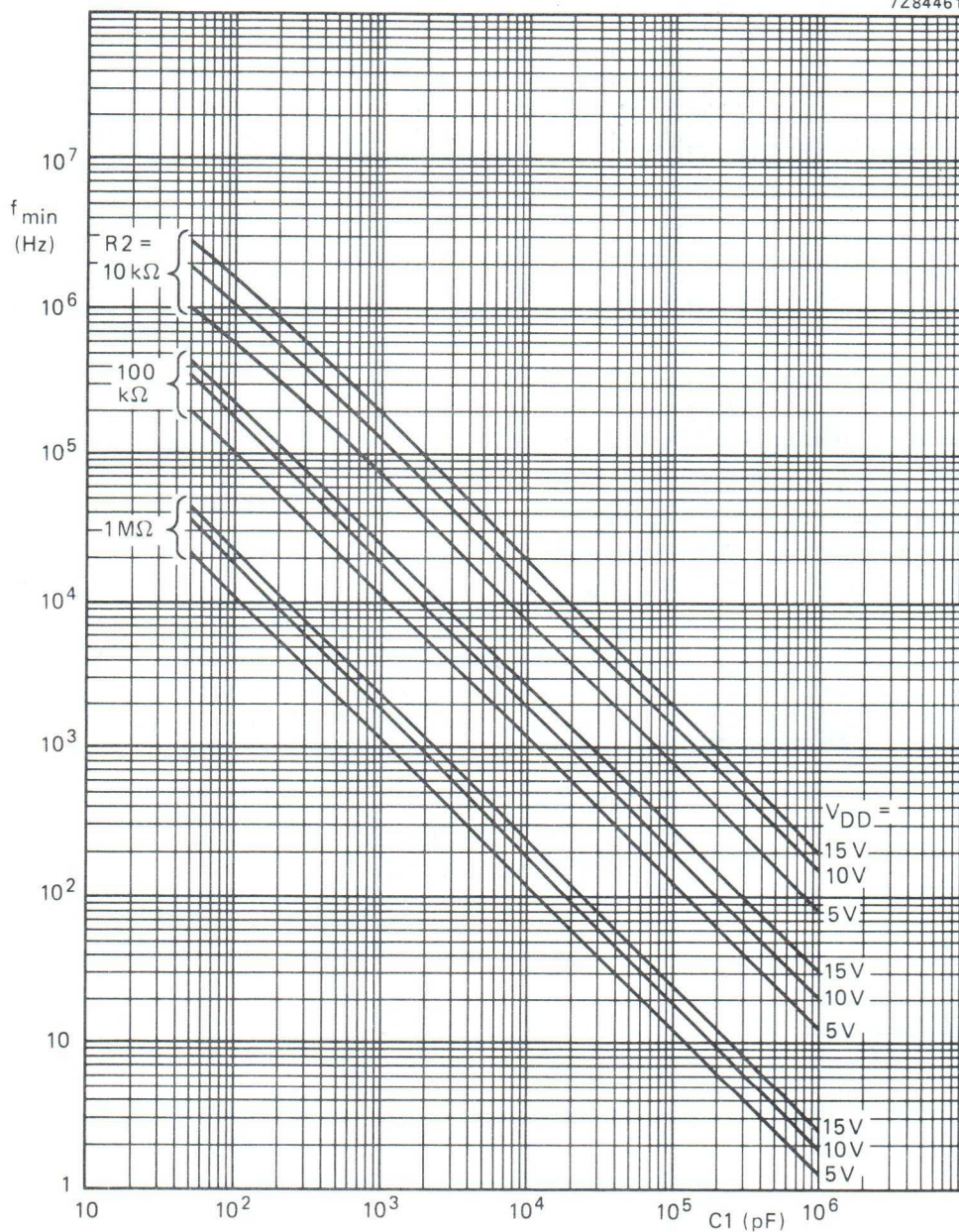
Fig. 8 Typical frequency offset as a function of capacitor C_1 ; T_{\text{amb}} = 25^\circ\text{C} ; V_{\text{COIN}} at V_{\text{SS}} ; \text{INH} at V_{\text{SS}} ; R_1 = \infty .
