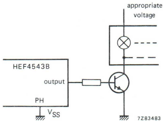
Fig. 9 Connection to incandescent display readout.
