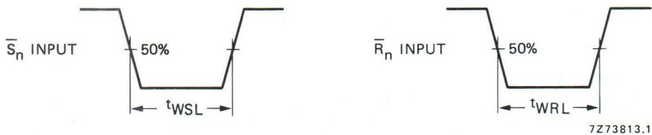
Fig. 5 Waveforms showing minimum \bar{S}_n and \bar{R}_n pulse widths.
