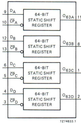
Quadruple 64-bit static shift register.
