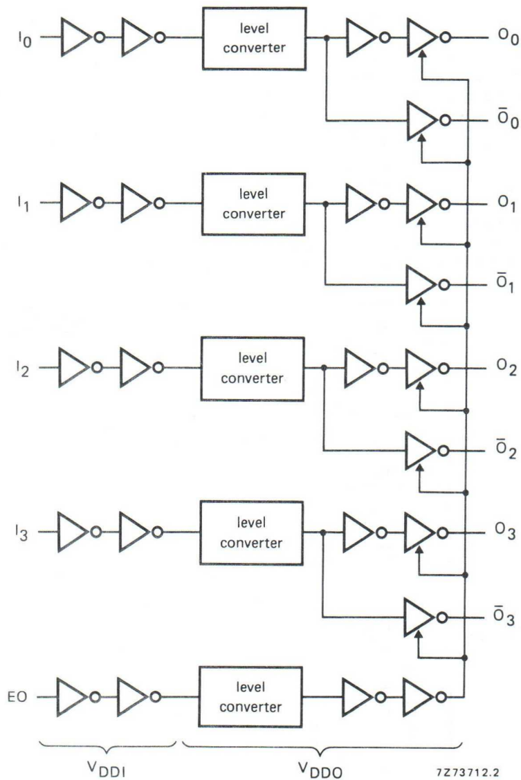
Fig. 3 Logic diagram.
