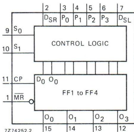
Fig. 1 Functional diagram.
