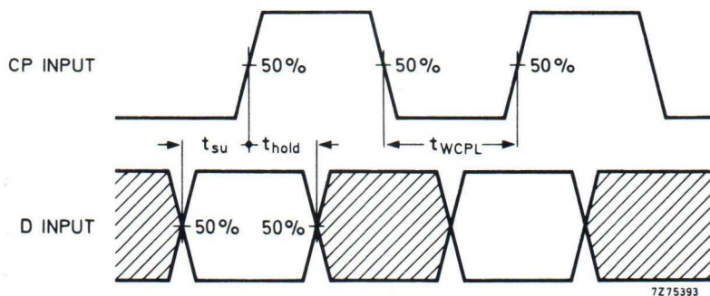
Fig. 5 Waveforms showing minimum clock pulse width, set-up time and hold time for CP and D.
