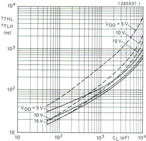
Fig. 7 Output transition times as a function of the load capacitance. —— t_{TLH} ; - - - - t_{THL} .
