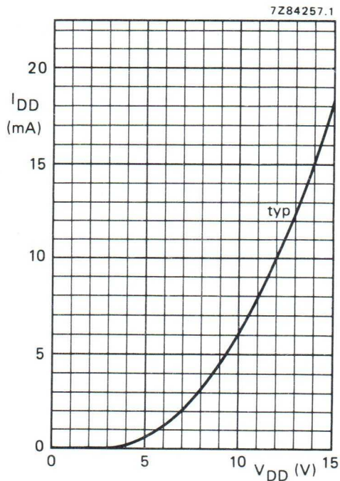
Fig. 7 Supply current as a function of supply voltage.
