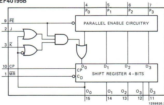
4-bit universal shift register.
