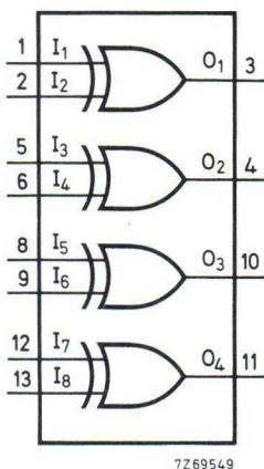
Fig. 1 Functional diagram.
