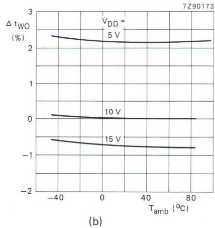
Fig. 7 Typical normalized change in output pulse width as a function of ambient temperature; 0% at V_{DD} = 10\text{ V} and T_{amb} = 25\text{ }^{\circ}\text{C} .
