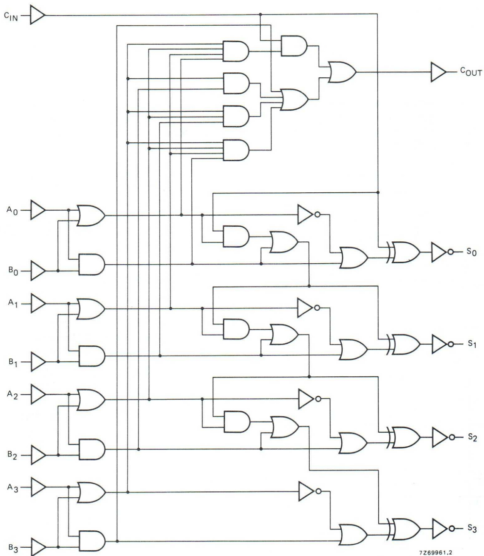
Fig. 3 Logic diagram.
