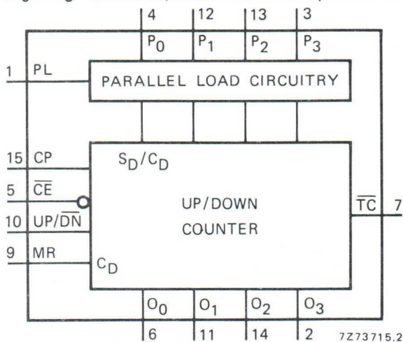
Fig. 1 Functional diagram.
