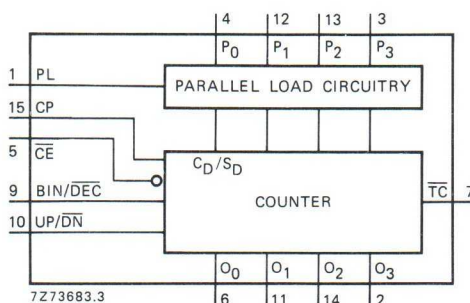
Fig. 1 Functional diagram.
