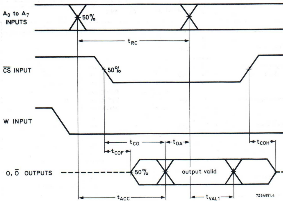
Fig. 3 Read cycle timing diagram.
