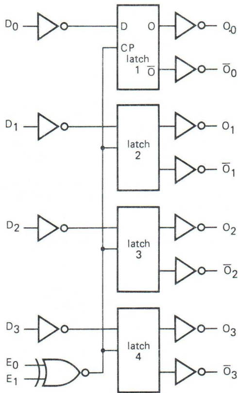
Fig. 3 Logic diagram.
