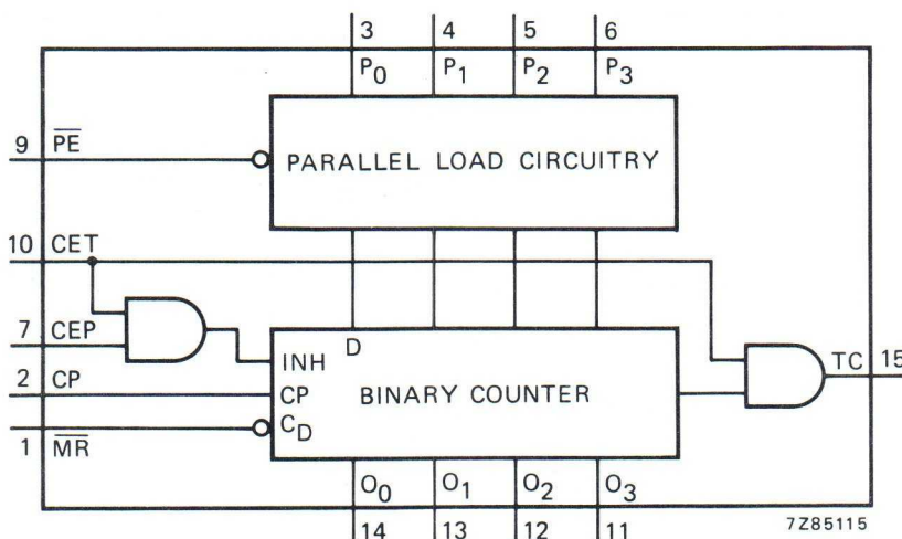
Fig. 1 Functional diagram.
