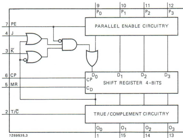
4-bit universal shift register.
