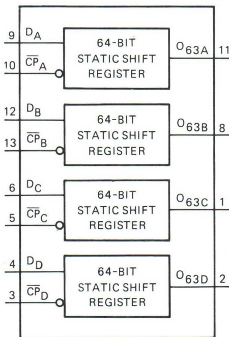
Fig. 1 Functional diagram. 7Z74633.1
