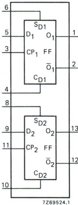
Fig. 1 Functional diagram.
