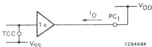
Fig. 12 Equivalent circuit for PC 1 sink current.
