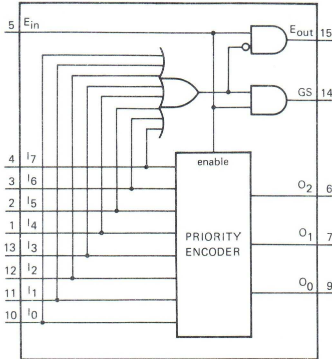
Fig. 1 Functional diagram.
