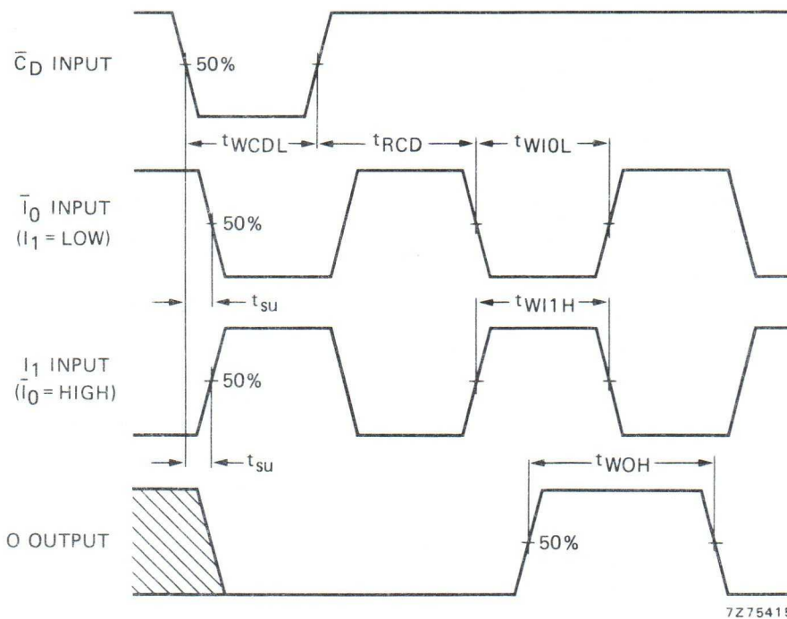
Fig. 5 Waveforms showing minimum \overline{I}_0 , I_1 and O pulse widths, set-up and recovery times. Set-up and recovery times are shown as positive values but may be specified as negative values.
