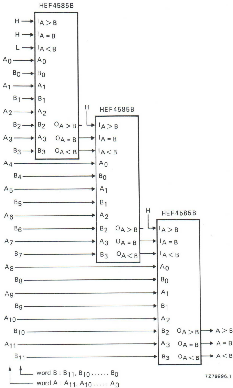
Fig. 4 Example of cascading comparators.
