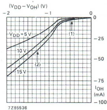
Fig. 4 Typical output source current characteristic.
