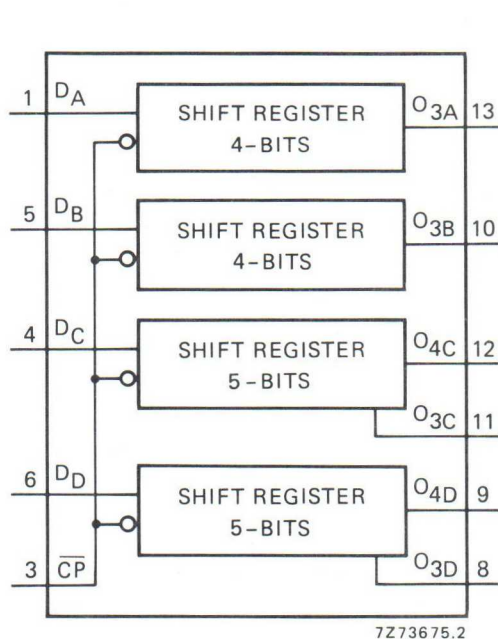
Fig. 1 Functional diagram.
