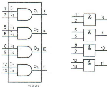
Quadrate 2-input AND gate.
