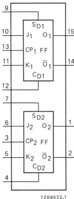
Fig. 1 Functional diagram.
