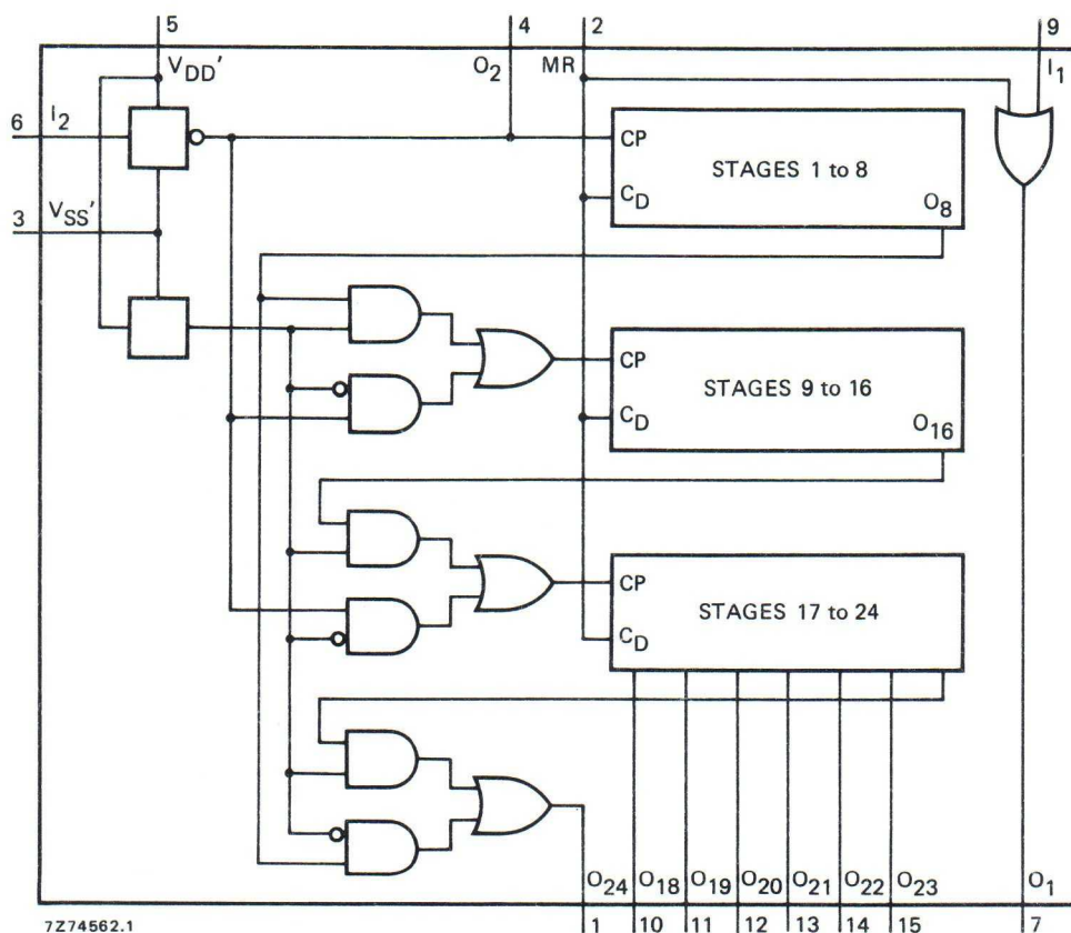
Fig. 1 Functional diagram.
