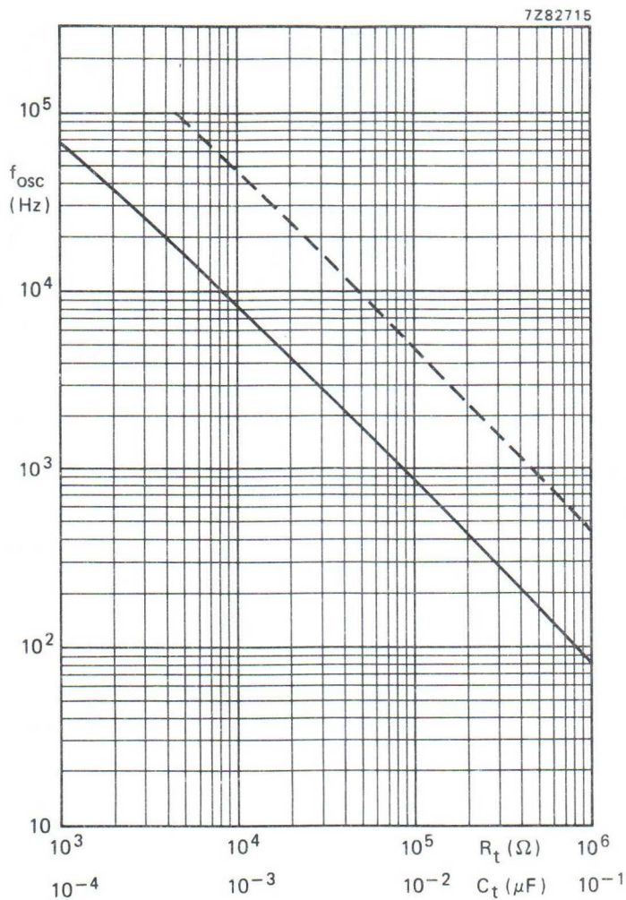
Fig. 5 RC oscillator frequency as a function of R_t and C_t at V_{DD} = 5 to 15 \text{ V} ; T_{amb} = 25^\circ \text{C} .
