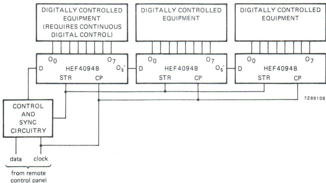
Fig. 5 Remote control holding register.
