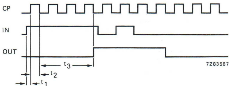
Fig. 7 Timing diagram for transient pulse suppression and pulse delaying mode; for t_1 , t_2 and t_3 see Fig. 5.
