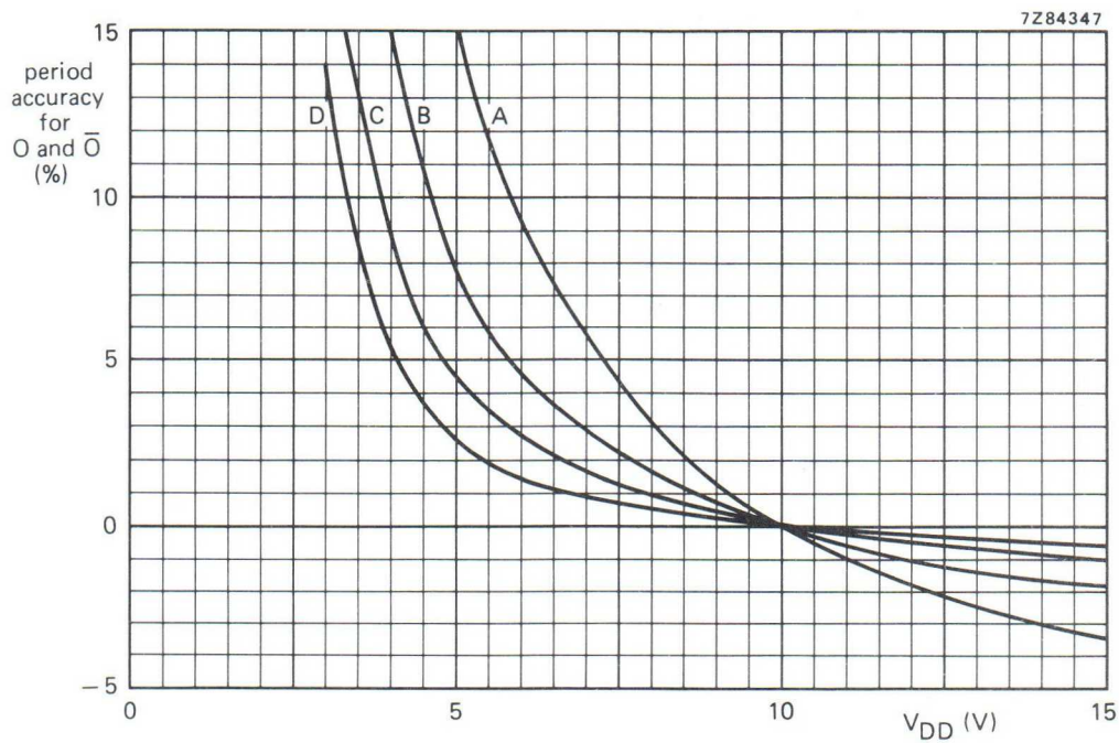
Fig. 6 Typical \bar{O} and \bar{O} period accuracy as a function of supply voltage; astable mode; T_{amb} = 25^\circ\text{C} .
