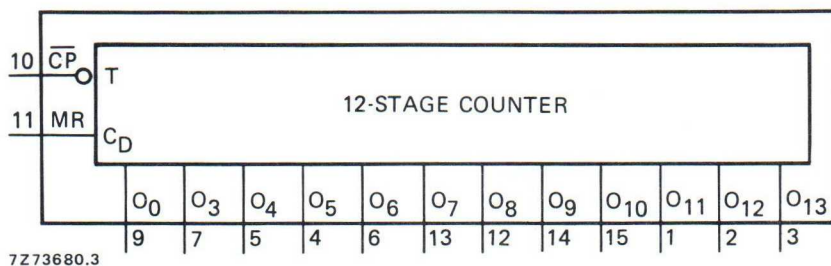
Fig. 1 Functional diagram.
