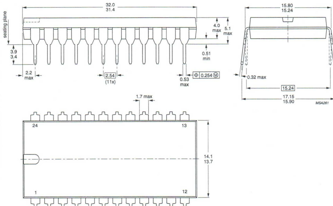
Fig.16 Plastic dual in-line package; 24 leads (600 mil); DIP24; SOT101-1.
