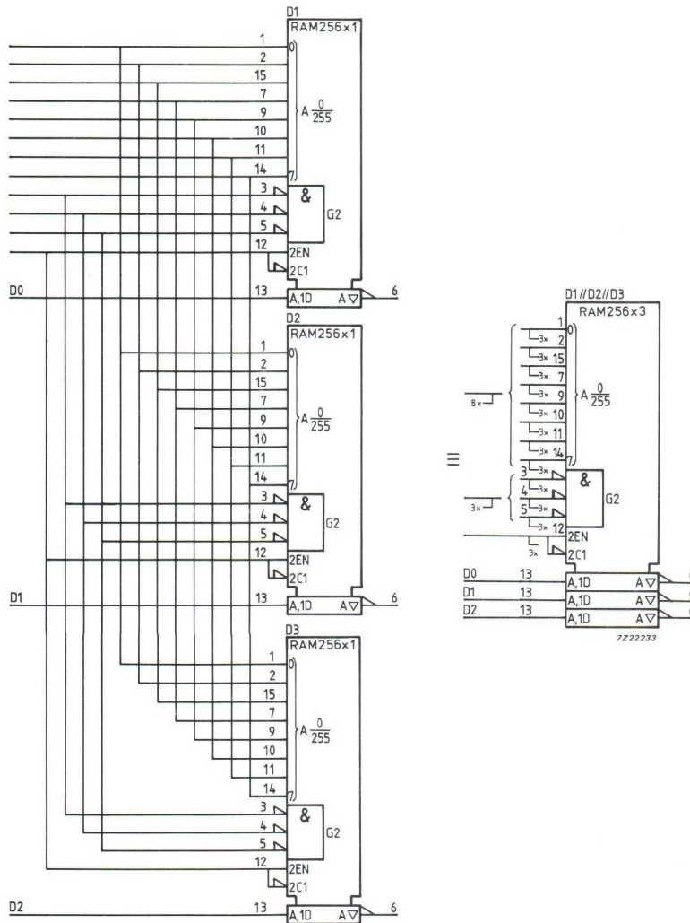
Fig. 47 Example of a multiple symbol showing three 256x1-bit RAMs connected to lengthen the word.
