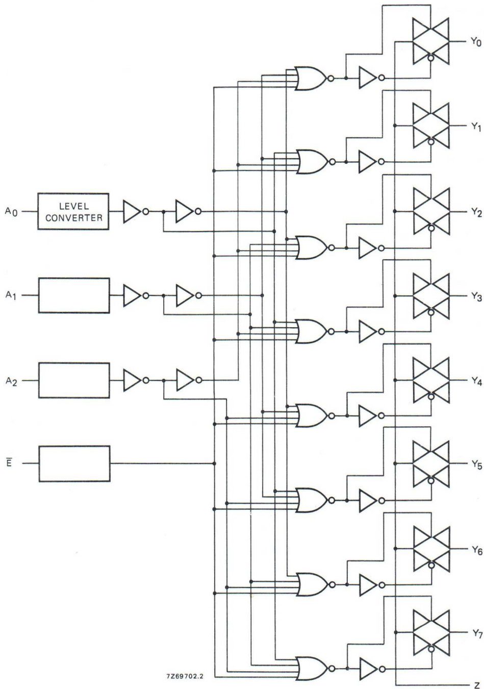
Fig. 4 Logic diagram.
