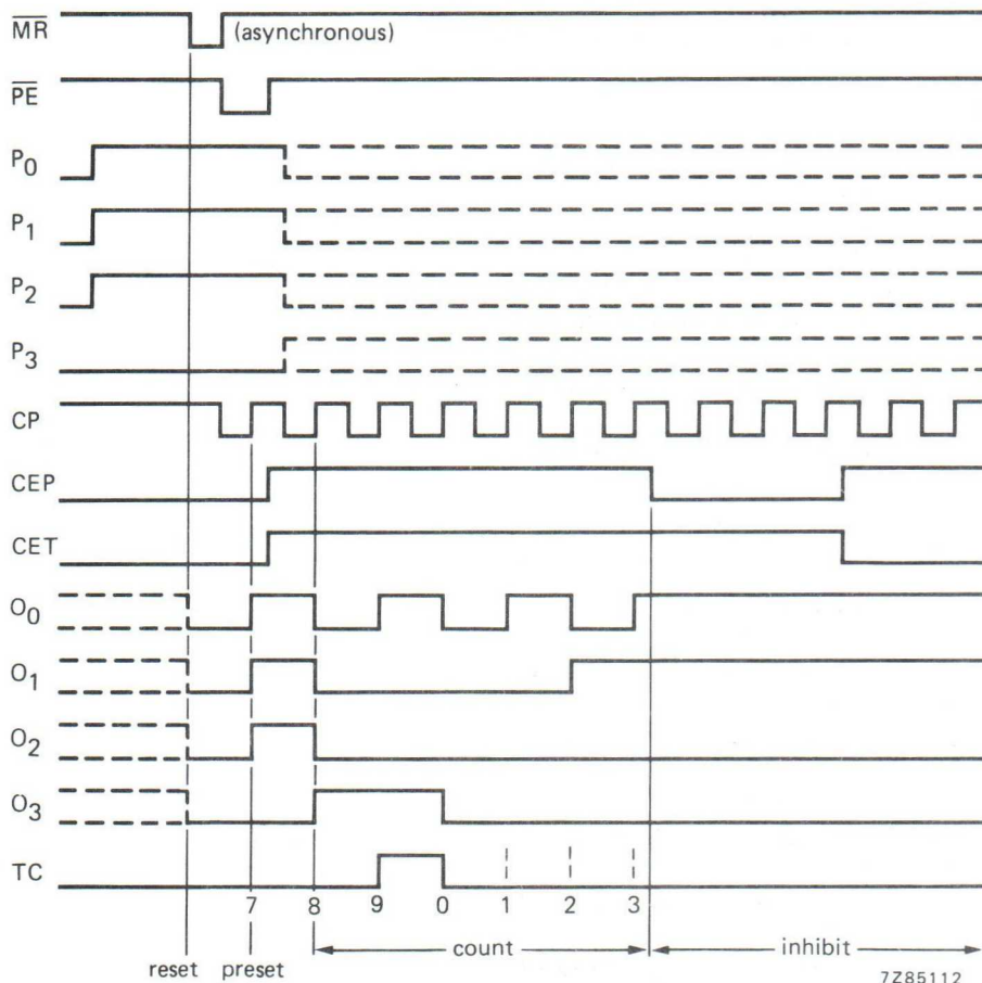
Fig. 9 Timing diagram.
