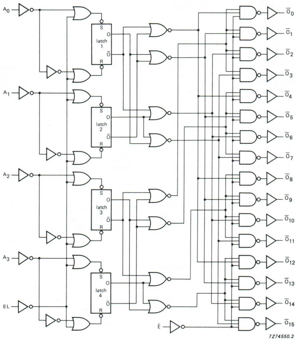
Fig. 3 Logic diagram.
