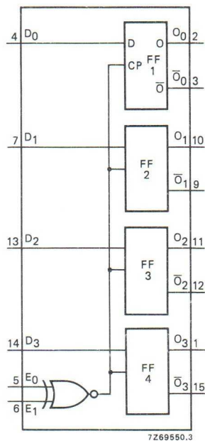
Quadruple D-latch.
