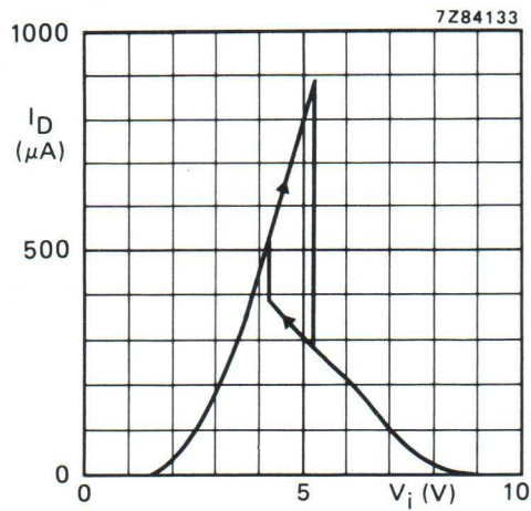
Fig. 7 Typical drain current as a function of input voltage; V_{DD} = 10\text{ V} ; T_{amb} = 25^\circ\text{C} .
