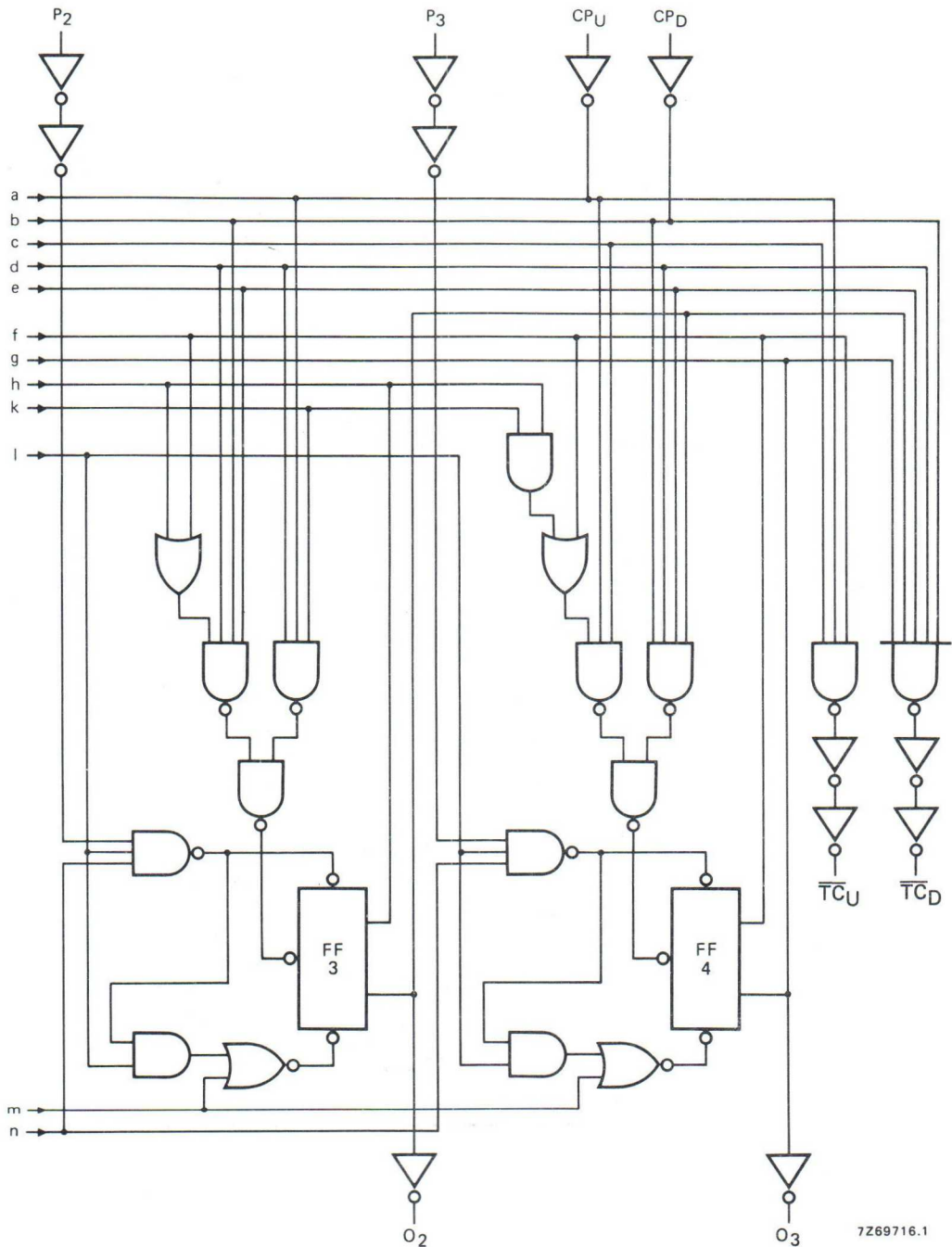
Fig. 3 Logic diagram (continued).
