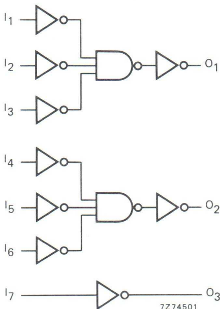
Fig. 3 Logic diagram.
