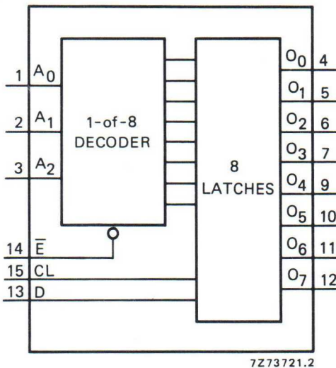
Fig. 1 Functional diagram.
