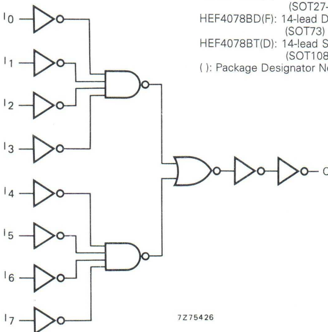
Fig. 3 Logic diagram.
