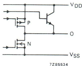
Fig. 6 Schematic diagram of output stage.
