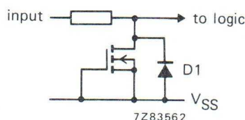
Fig. 14 The input protection for the HEF4049B and HEF4050B.
