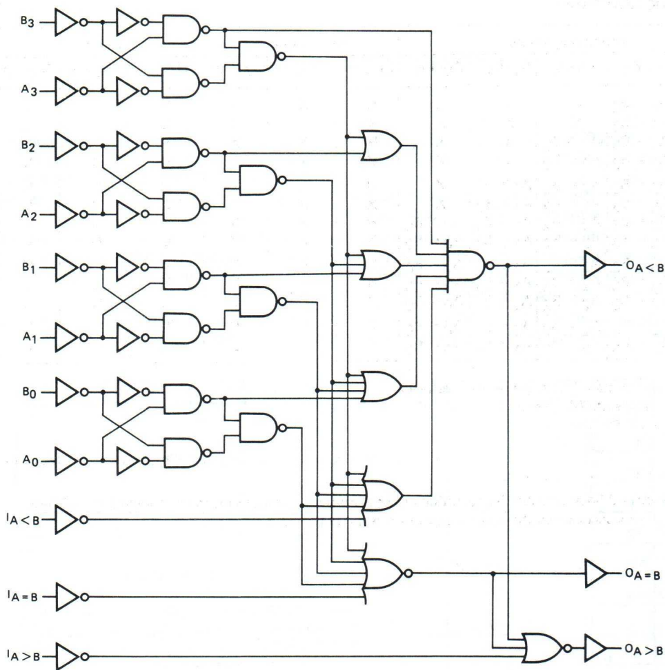
Fig. 3 Logic diagram.
