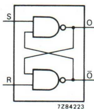
Fig. 4 Logic diagram (one latch).
