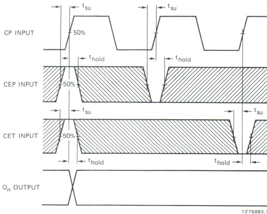
Fig. 6 Waveforms showing set-up times and hold times for CEP and CET inputs.
