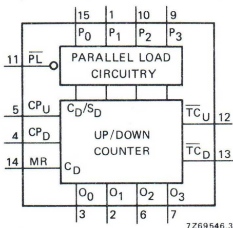
Fig. 1 Functional diagram.
