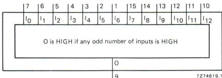
Fig. 1 Functional diagram.
