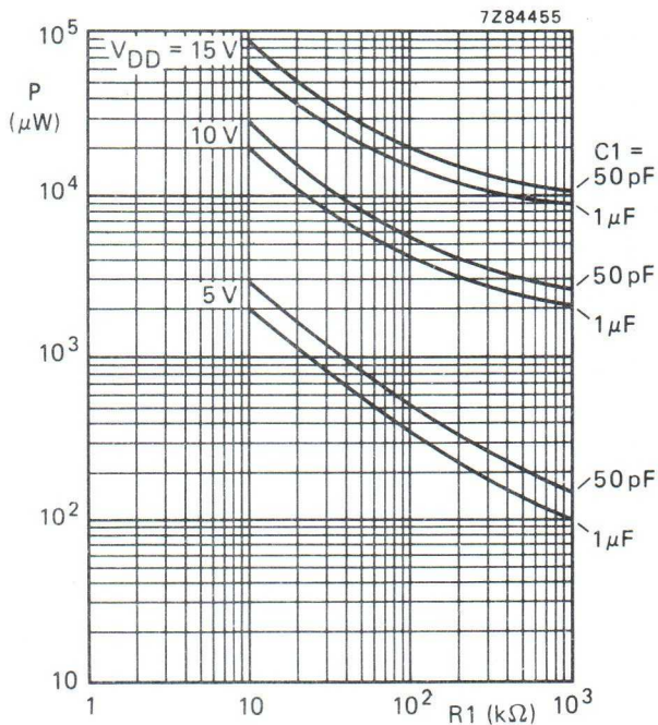
Fig. 10 Power dissipation as a function of R_1 ; R_2 = \infty ; V_{COIN} at \frac{1}{2} V_{DD} ; C_L = 50 pF .
