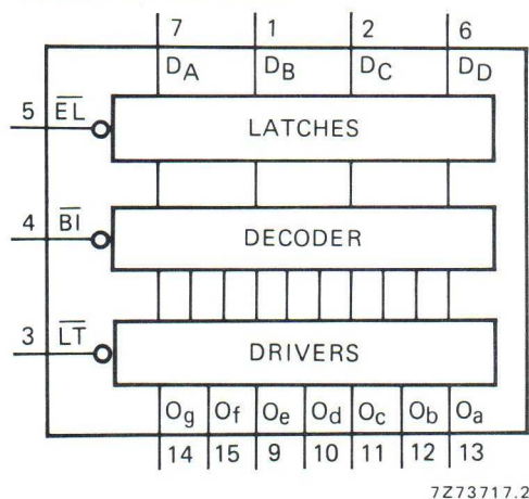
Fig. 1 Functional diagram.
