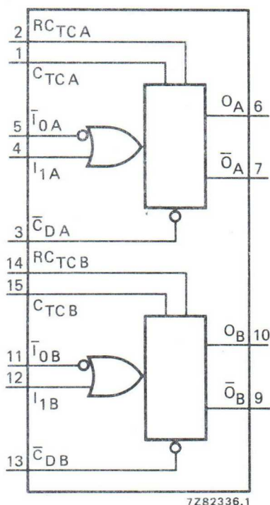
Fig. 1 Functional diagram.
