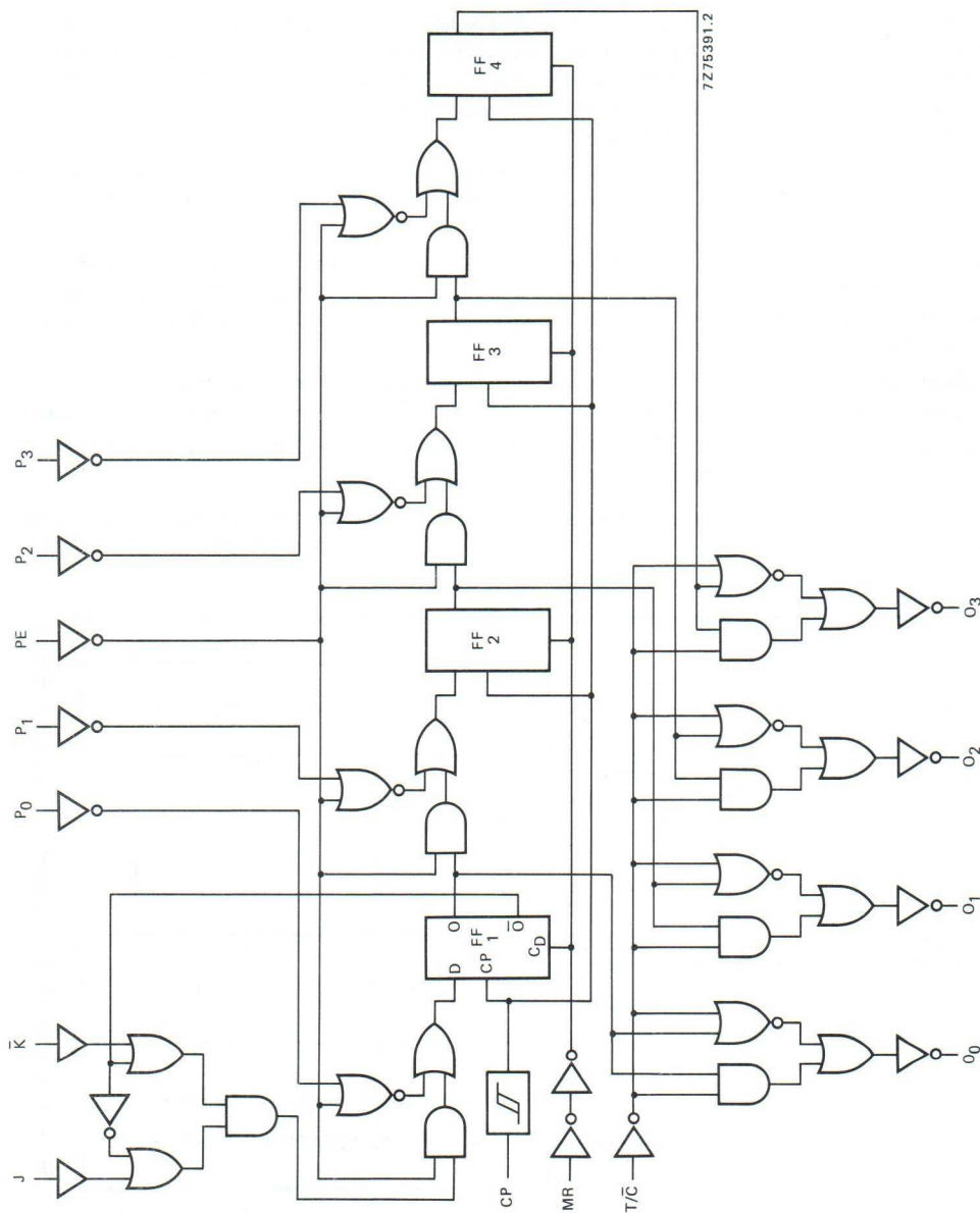
Fig. 2 Logic diagram.
