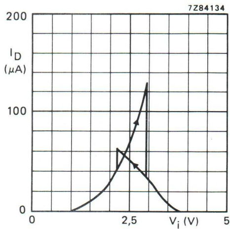
Fig. 6 Typical drain current as a function of input voltage; V_{DD} = 5\text{ V} ; T_{amb} = 25^\circ\text{C} .
