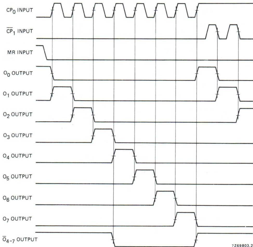
Fig. 6 Timing diagram.
