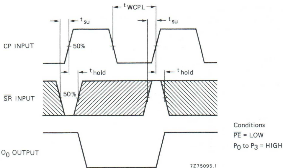
Fig. 5 Waveforms showing set-up and hold times for \overline{SR} input and minimum CP pulse width.
