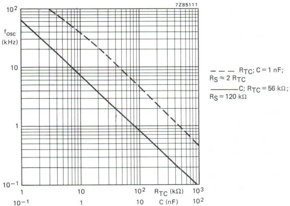
Fig. 8 Oscillator frequency as a function of R_{TC} and C ; V_{DD} = 10 \text{ V} ; test circuit is Fig. 7.
