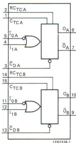
Dual monostable multivibrator.
