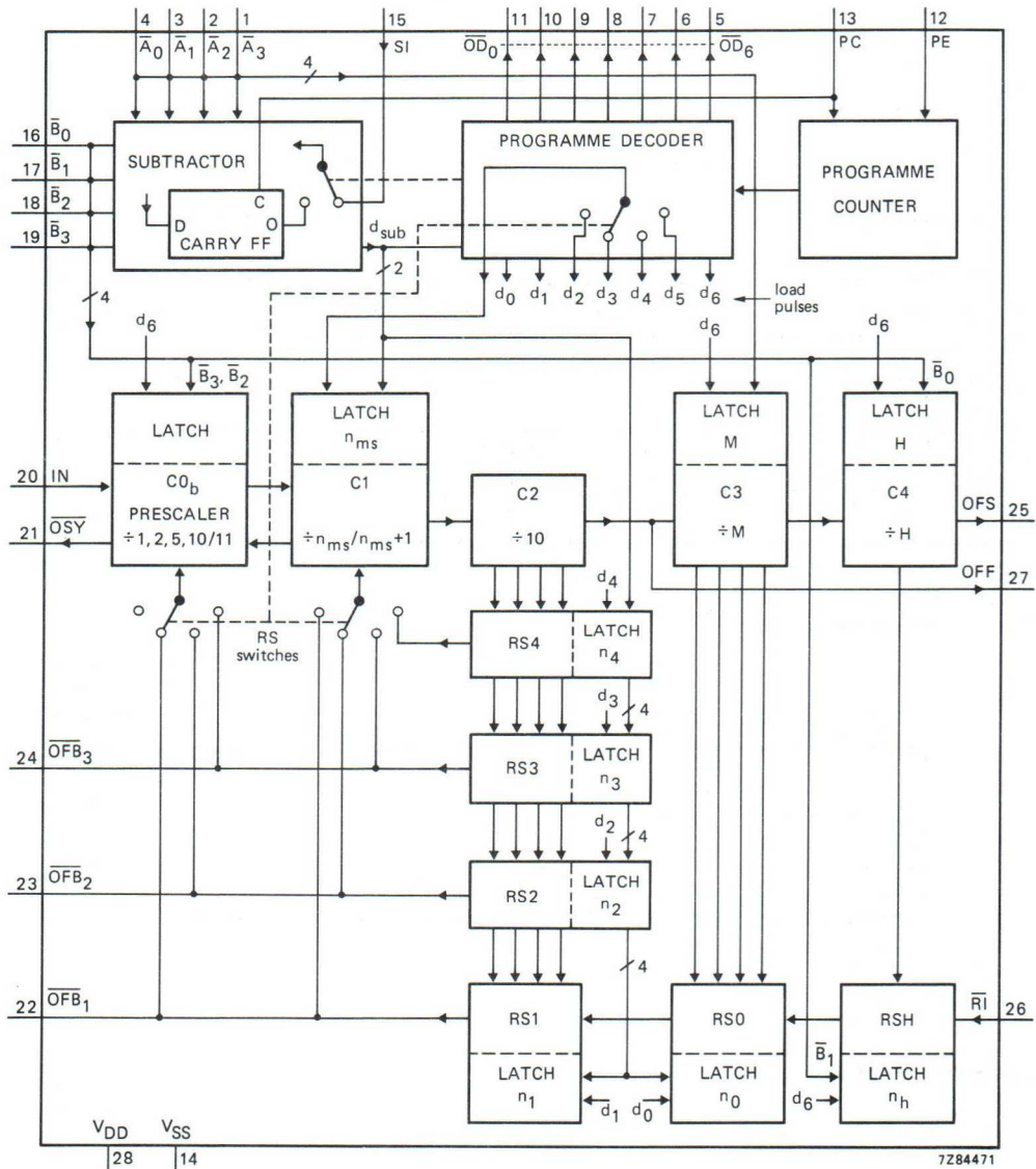
Fig. 2 Block diagram.
