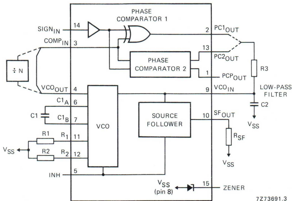
Fig. 1 Functional diagram.
