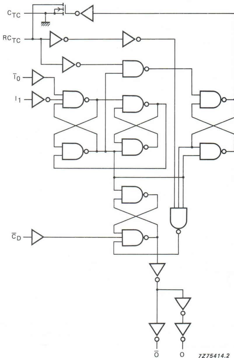
Fig. 3 Logic diagram (one monostable multivibrator).
