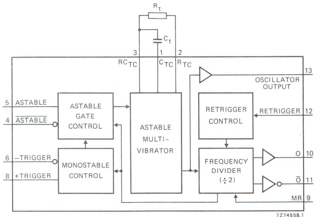
Fig. 1 Functional diagram.
