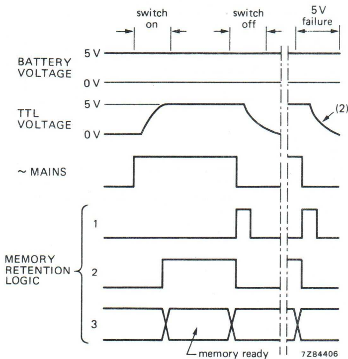
Fig. 10 Using a thyristor to ensure a rapid fall of interface supply at switch-off or supply failure.
