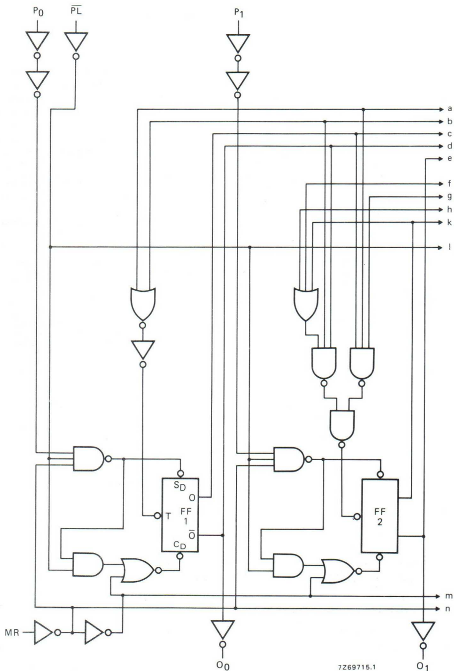
Fig. 3 Logic diagram (continued on next page).
