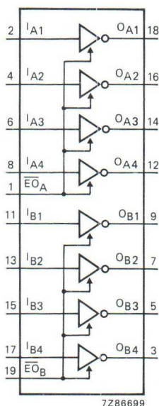
Fig. 1 Functional diagram.
