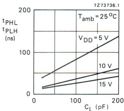
Fig. 7 Positive and negative-going propagation delay as functions of load capacitance for the HEF4011B.
