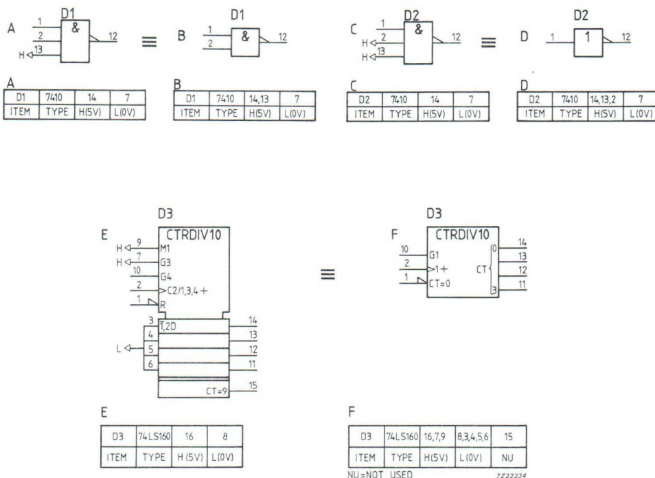
Fig. 38 Examples of Rule 1.
