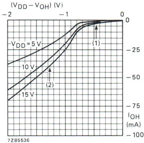
Fig. 4 Typical output source current characteristic.
