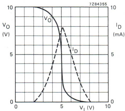
Fig. 4 Typical drain current I_D and output voltage V_O as functions of input voltage; V_{DD} = 10\text{ V} ; T_{amb} = 25\text{ }^{\circ}\text{C} .
