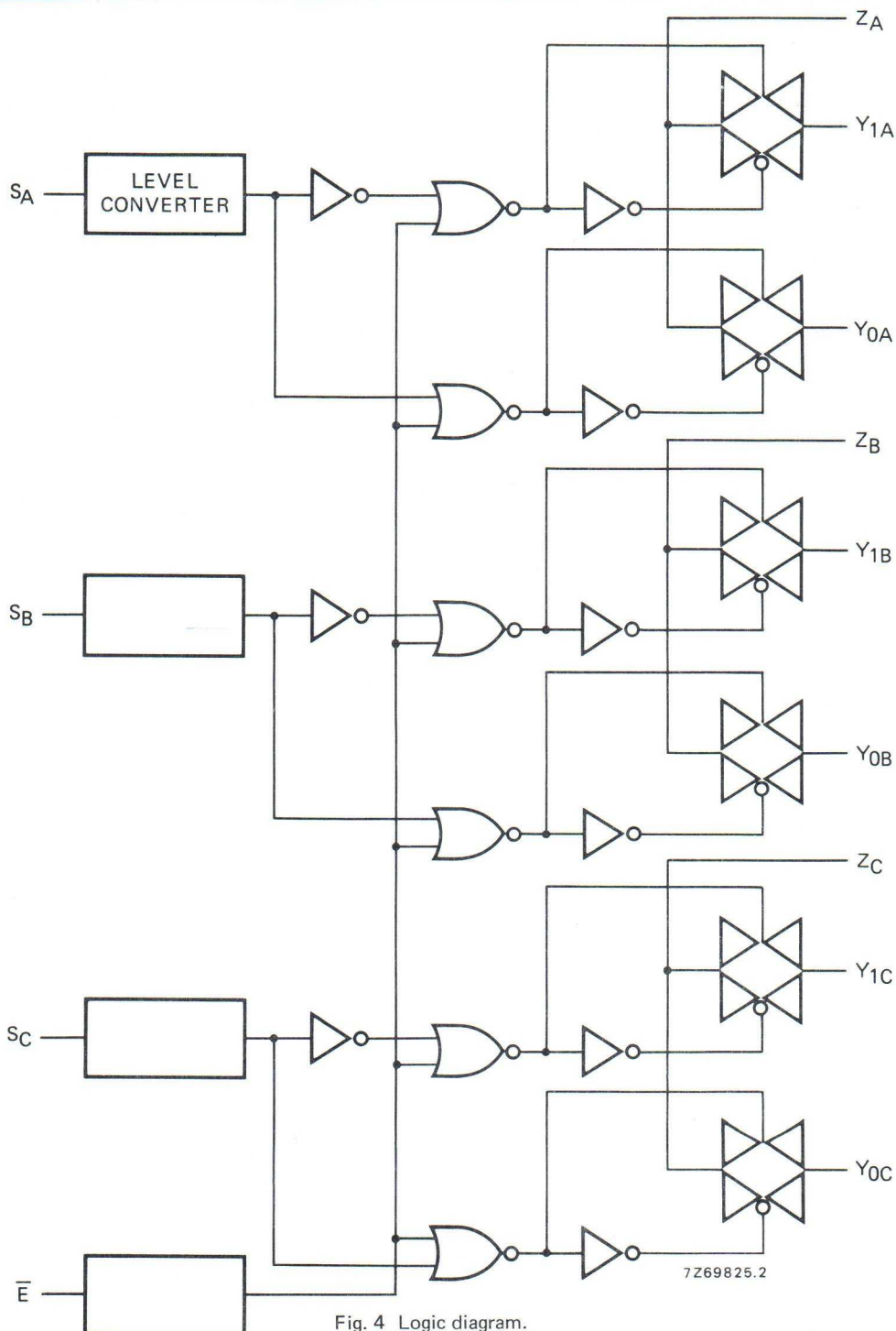
Fig. 4 Logic diagram.
