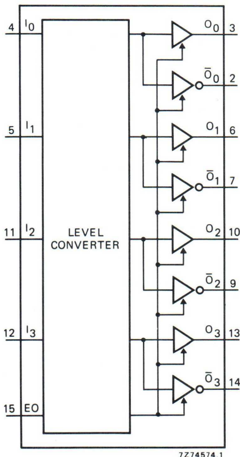
Fig. 1 Functional diagram.
