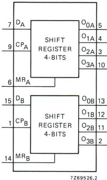
Fig. 1 Functional diagram.
