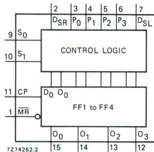
4-bit bidirectional universal shift register.
