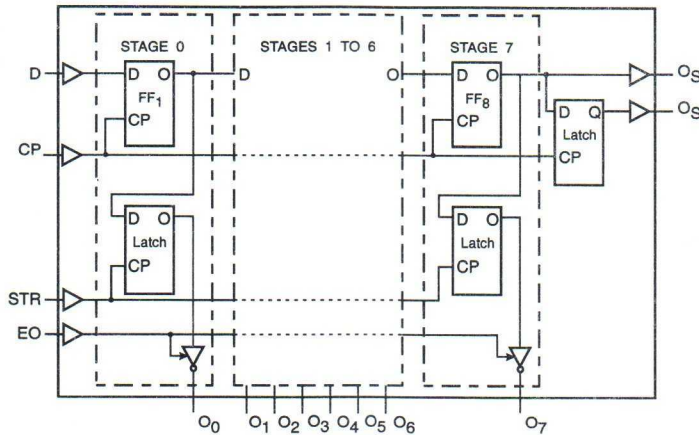
Fig.3 Logic diagram.
