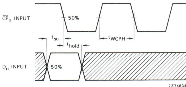
Fig. 4 Waveforms showing minimum clock pulse width, set-up and hold times for D to \overline{CP} . Set-up and hold times are shown as positive values but may be specified as negative values.
