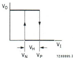
Fig. 4 Transfer characteristic.
