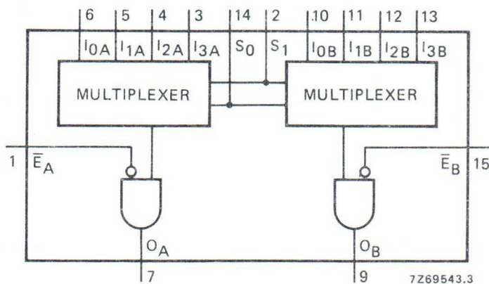
Fig. 1 Functional diagram.
