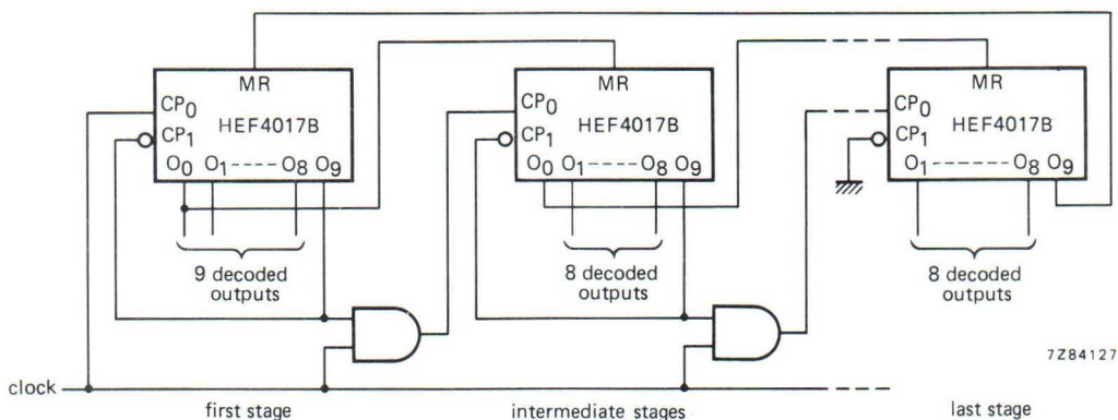
Fig. 7 Counter expansion.
