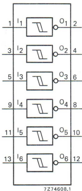
Fig. 1 Functional diagram.
