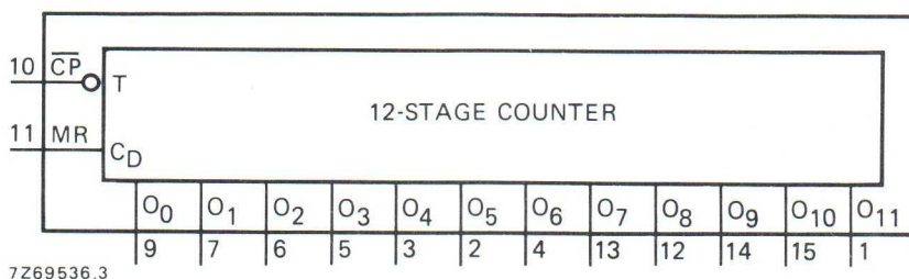
Fig. 1 Functional diagram.
