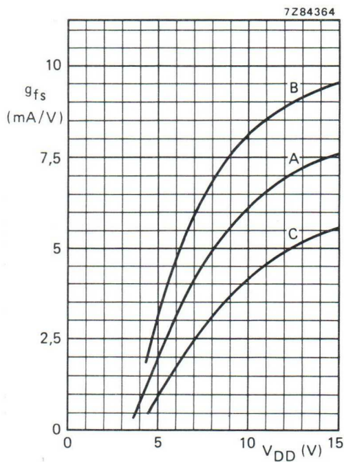
Fig. 8 Typical forward transconductance g_{fs} as a function of the supply voltage at T_{\text{amb}} = 25^\circ\text{C} .
