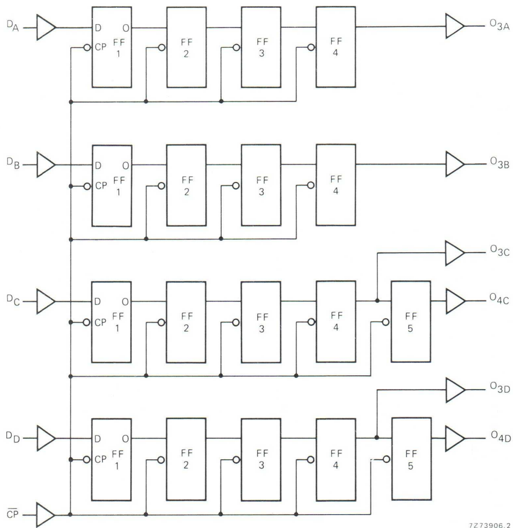
Fig. 3 Logic diagram.
