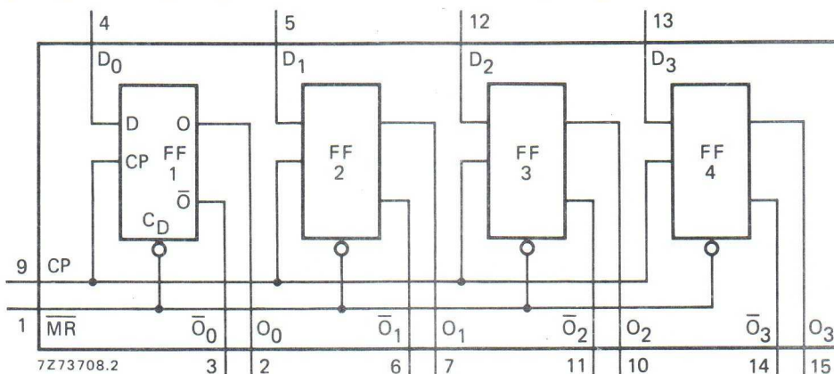
Fig. 1 Functional diagram.
