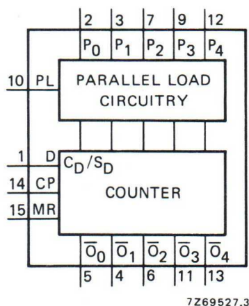
Fig. 1 Functional diagram.
