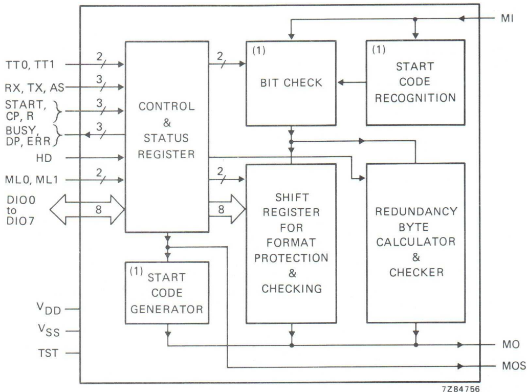
Fig. 2 Block diagram.
