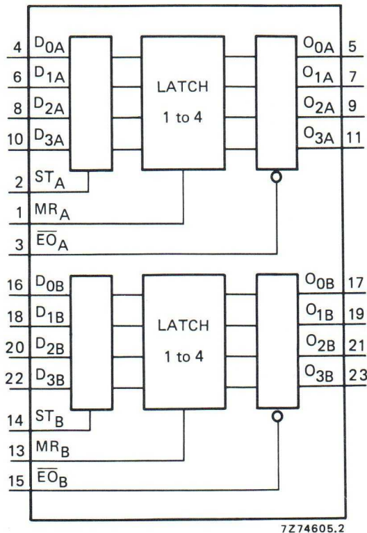
Fig. 1 Functional diagram.
