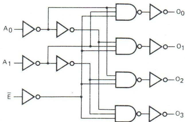
Fig. 3 Logic diagram (one decoder/multiplexer).
