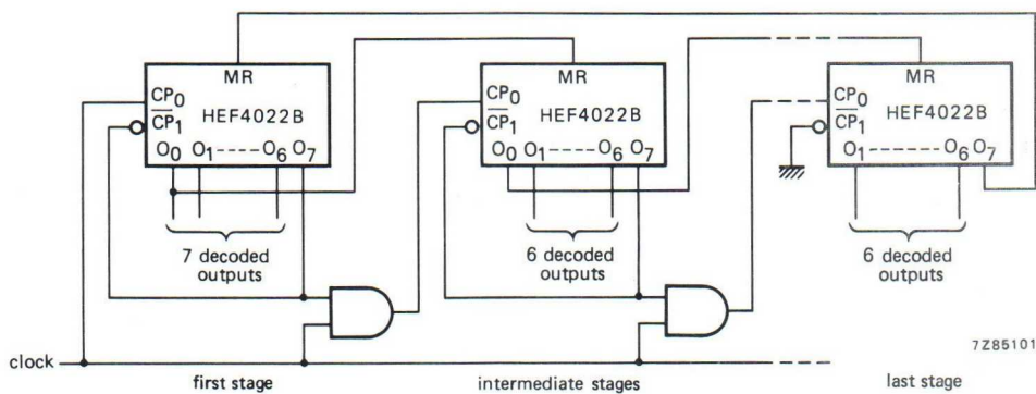
Fig. 7 Counter expansion.
