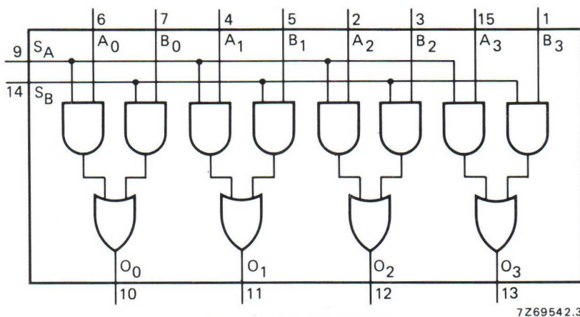
Fig. 1 Functional diagram.
