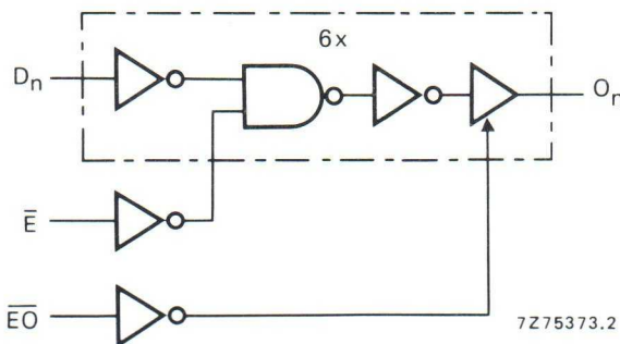
Fig. 3 Logic diagram.
