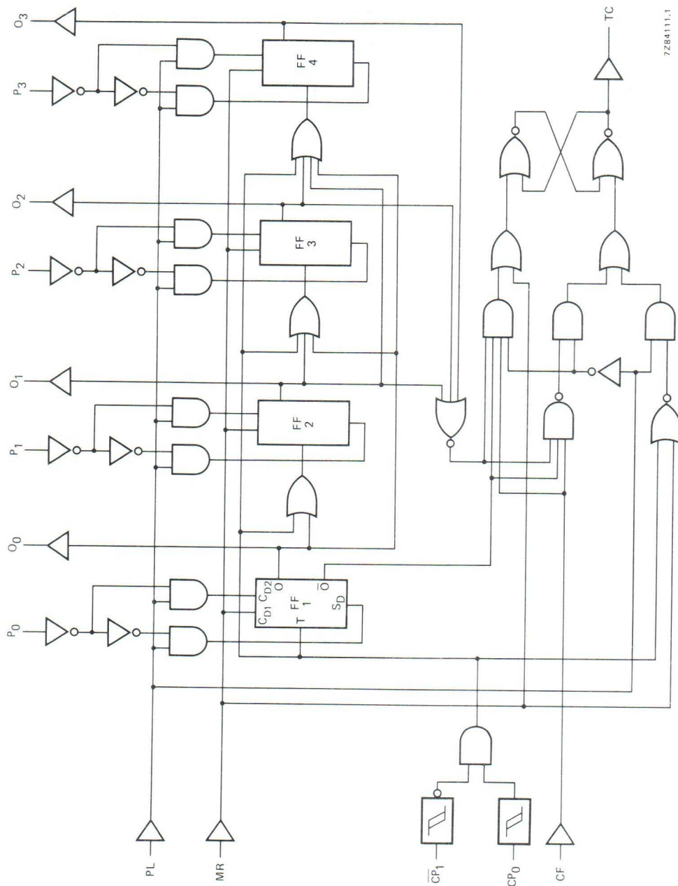
Fig. 4 Logic diagram.
