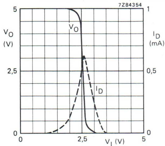
Fig. 3 Typical drain current I_D and output voltage V_O as functions of input voltage; V_{DD} = 5\text{ V} ; T_{amb} = 25\text{ }^{\circ}\text{C} .
