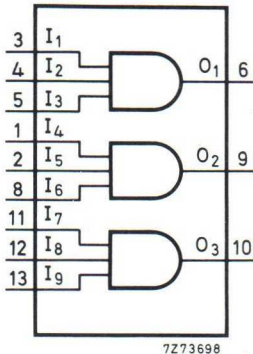
Fig.1 Functional diagram.
