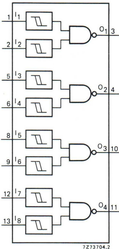
Fig. 1 Functional diagram.
