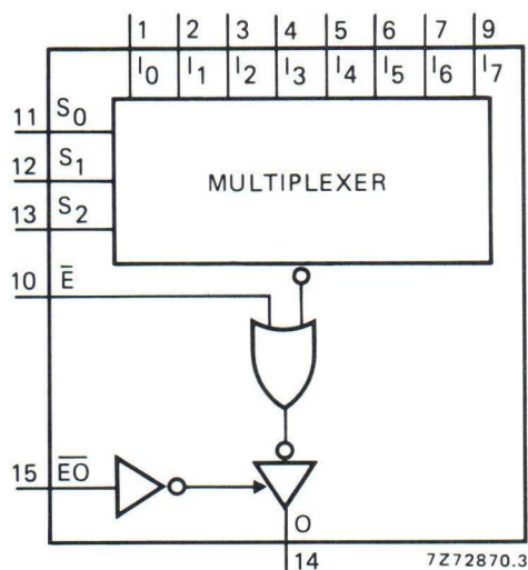
Fig. 1 Functional diagram.
