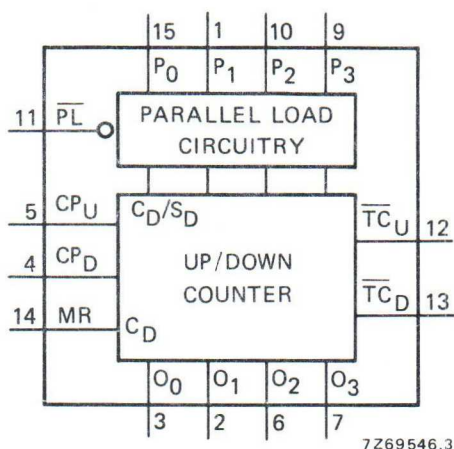
Fig. 1 Functional diagram.
