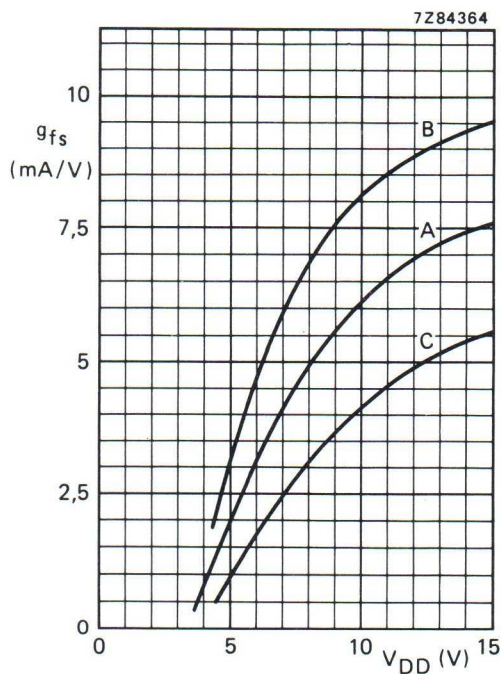
Fig. 10 Typical forward transconductance g_{fs} as a function of the supply voltage at T_{\text{amb}} = 25^\circ\text{C} .
