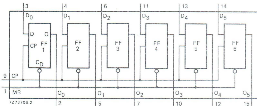
Fig. 1 Functional diagram.
