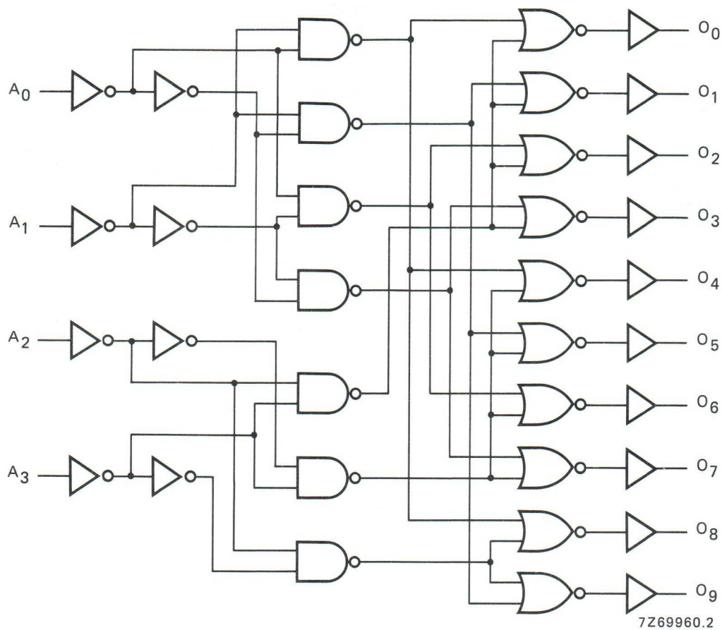
Fig. 3 Logic diagram.
