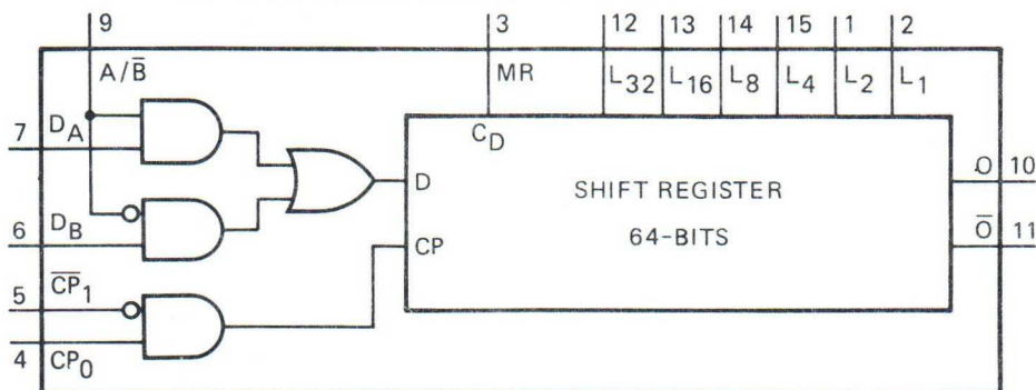
Fig. 1 Functional diagram.
