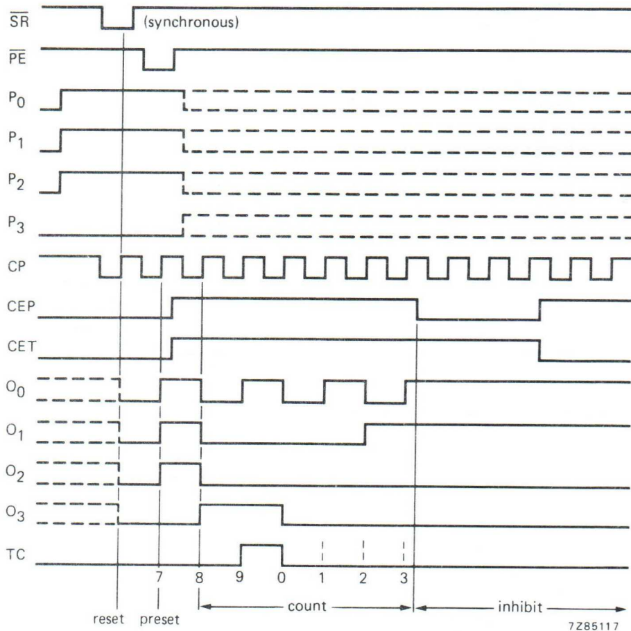
Fig. 9 Timing diagram.
