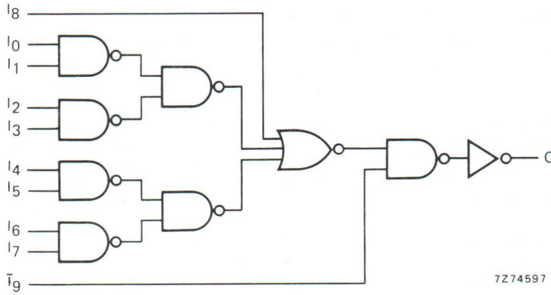
Fig. 3 Logic diagram.
