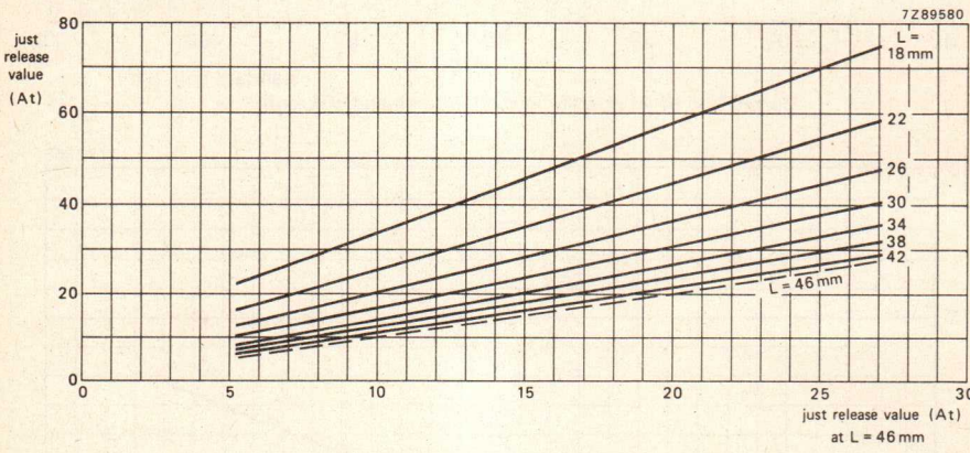
Just release values at various overall lengths compared with standard length of 46 mm.
