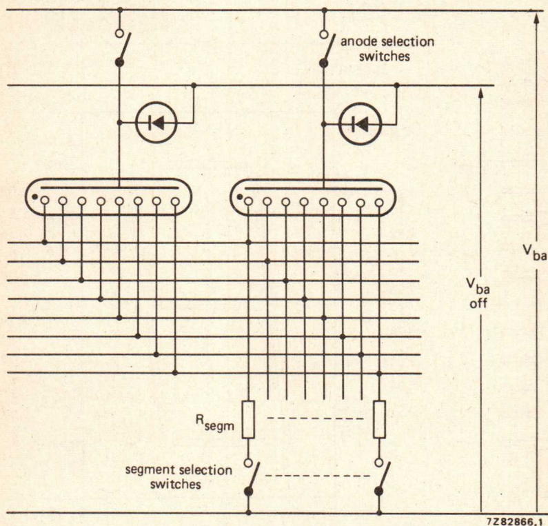
Fig. 2 Dynamic operation.
