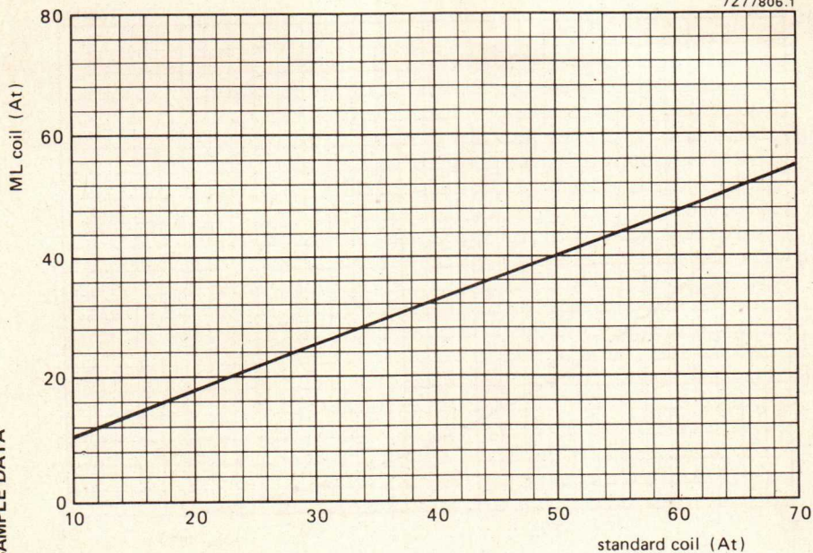
Correlation of At operate in standard coil and MIL coil.
