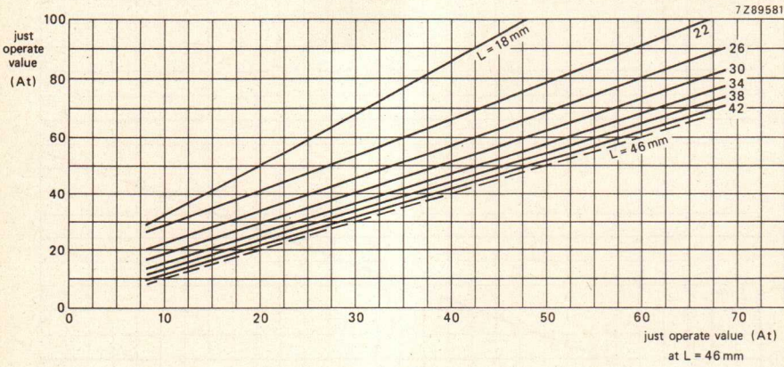
Just operate values at various overall lengths compared with standard length of 46 mm.
