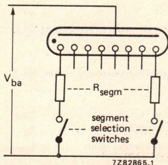
Fig. 1 Static operation.
