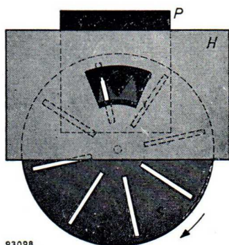
Fig. 8. Schematic representation of the optical siren (see photo on title page). A beam of light emitted by light-source W is concentrated on a photomultiplier tube F by a lens L . Situated in the beam is a holder H containing a sheet of paper P in which a waveform has been cut out, and behind which rotates a disc S driven by a motor M . As the disc rotates the pattern is successively scanned by narrow radial slits in the disc, and the light passing through the slit varies in accordance with the ordinate of the pattern. The photoelectric current in F varies in the same rhythm and is passed via an amplifier to the loudspeaker U .
