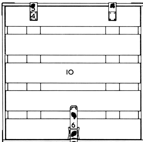
PLAN SHOWING LID CLOSED
