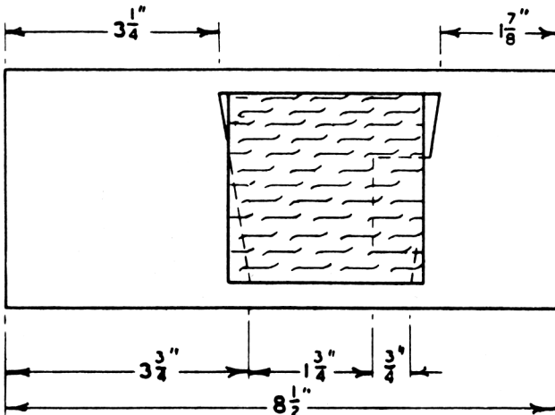
PLAN OF LID.
