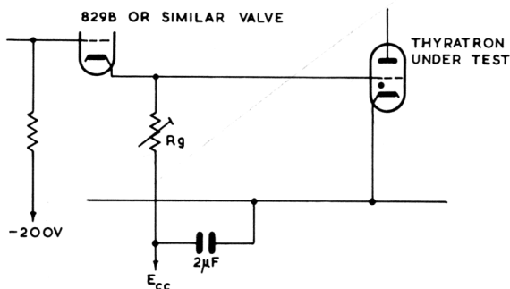
FIG. 4 OPERATION CIRCUIT WITH BIAS
