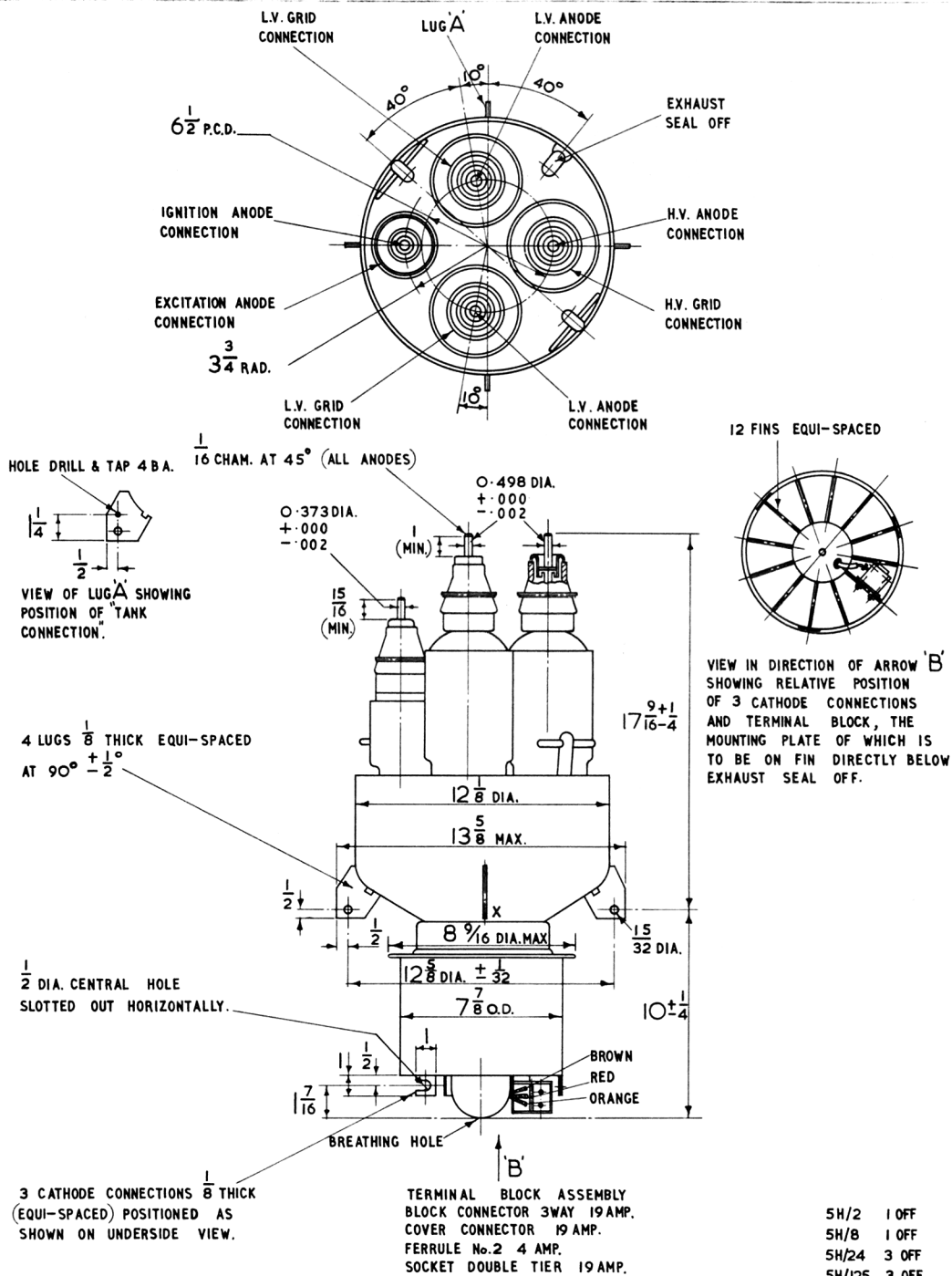
CV2455 OUTLINE DRAWING
