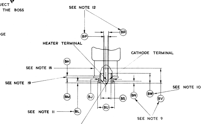
TERMINAL ASSEMBLY
