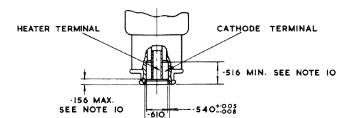
ALTERNATIVE TERMINAL ASSEMBLY I (NOTE 20)
