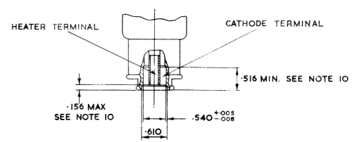
ALTERNATIVE TERMINAL ASSEMBLY I (NOTE 20)
