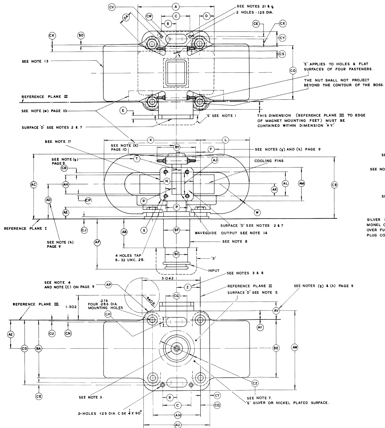
ALTERNATIVE TERMINAL ASSEMBLY II (NOTE 20)
