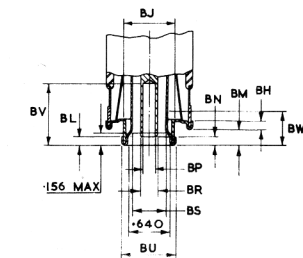
ALTERNATIVE TERMINAL ASSEMBLY II (NOTE 20)
