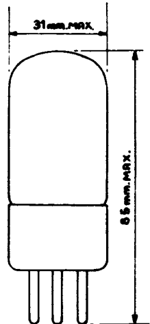
BRITISH 4-PIN BASE
