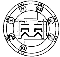
BOTTOM VIEW MINIATURE BUTTON 7 PIN BASE 68T
