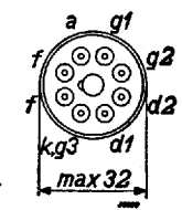
Fig. 2 Arrangement and sequence of connections.
