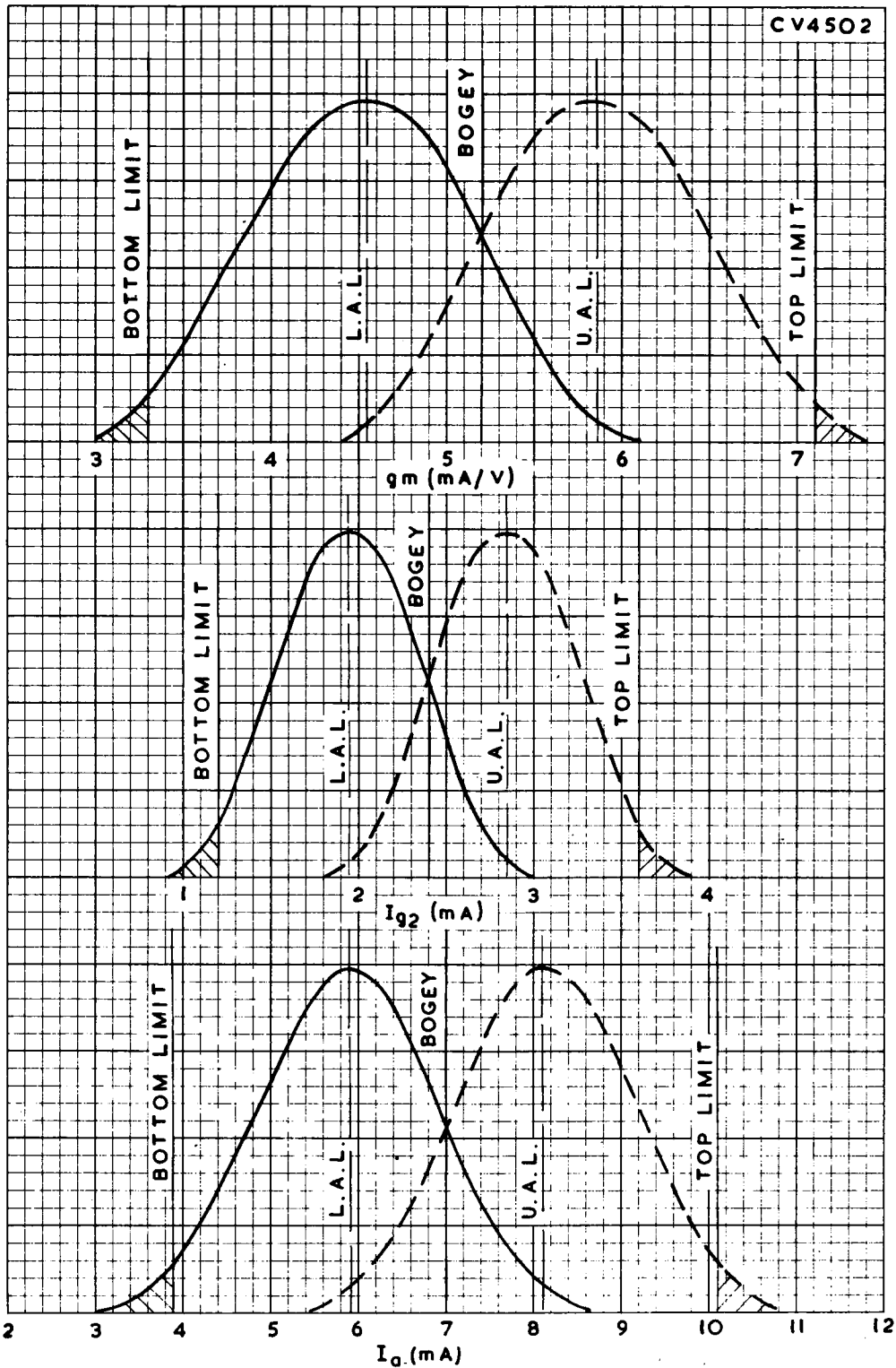
LIMITING DISTRIBUTIONS OF MAJOR CHARACTERISTICS
