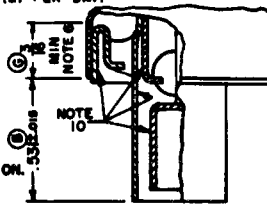
ALTERNATE CONSTRUCTION OF CATHODE END OF TUBE
